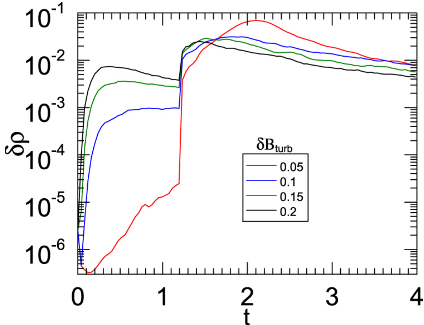
Figure 7. from The Parametric Decay Instability of Alfvén Waves in Turbulent Plasmas and the Applications in the Solar Wind null 2017 APJ 842 63 doi:10.3847/1538-4357/aa71b6 https://dx.doi.org/10.3847/1538-4357/aa71b6 © 2017. The American Astronomical Society. All rights reserved.
