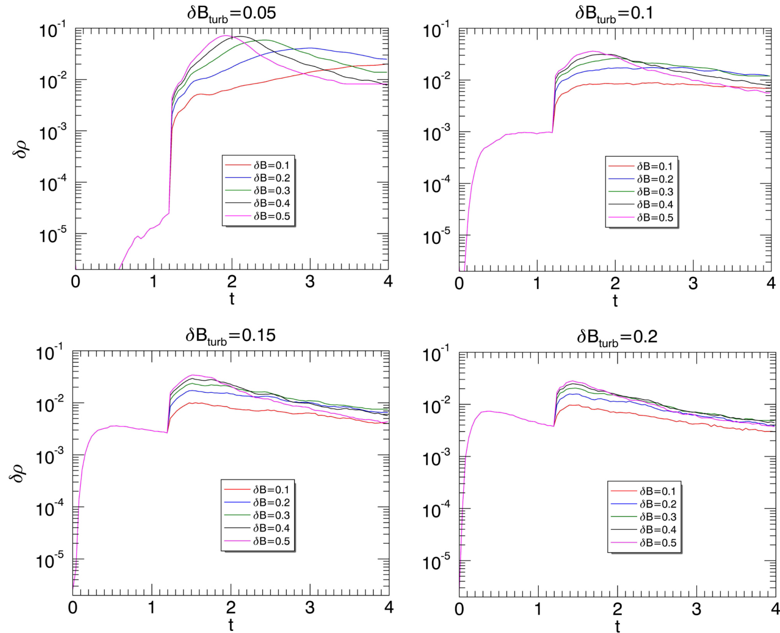
Figure 6. from The Parametric Decay Instability of Alfvén Waves in Turbulent Plasmas and the Applications in the Solar Wind null 2017 APJ 842 63 doi:10.3847/1538-4357/aa71b6 https://dx.doi.org/10.3847/1538-4357/aa71b6 © 2017. The American Astronomical Society. All rights reserved.
