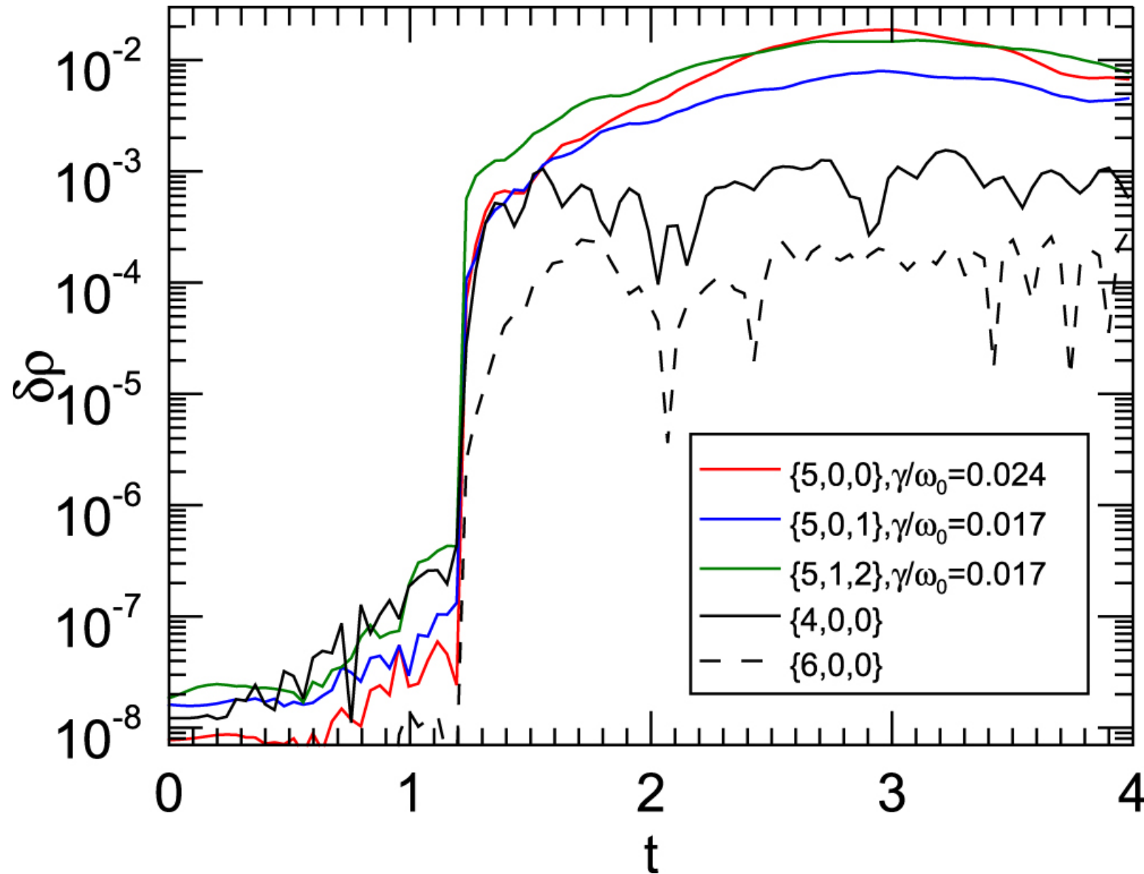
Figure 4. from The Parametric Decay Instability of Alfvén Waves in Turbulent Plasmas and the Applications in the Solar Wind null 2017 APJ 842 63 doi:10.3847/1538-4357/aa71b6 https://dx.doi.org/10.3847/1538-4357/aa71b6 © 2017. The American Astronomical Society. All rights reserved.
