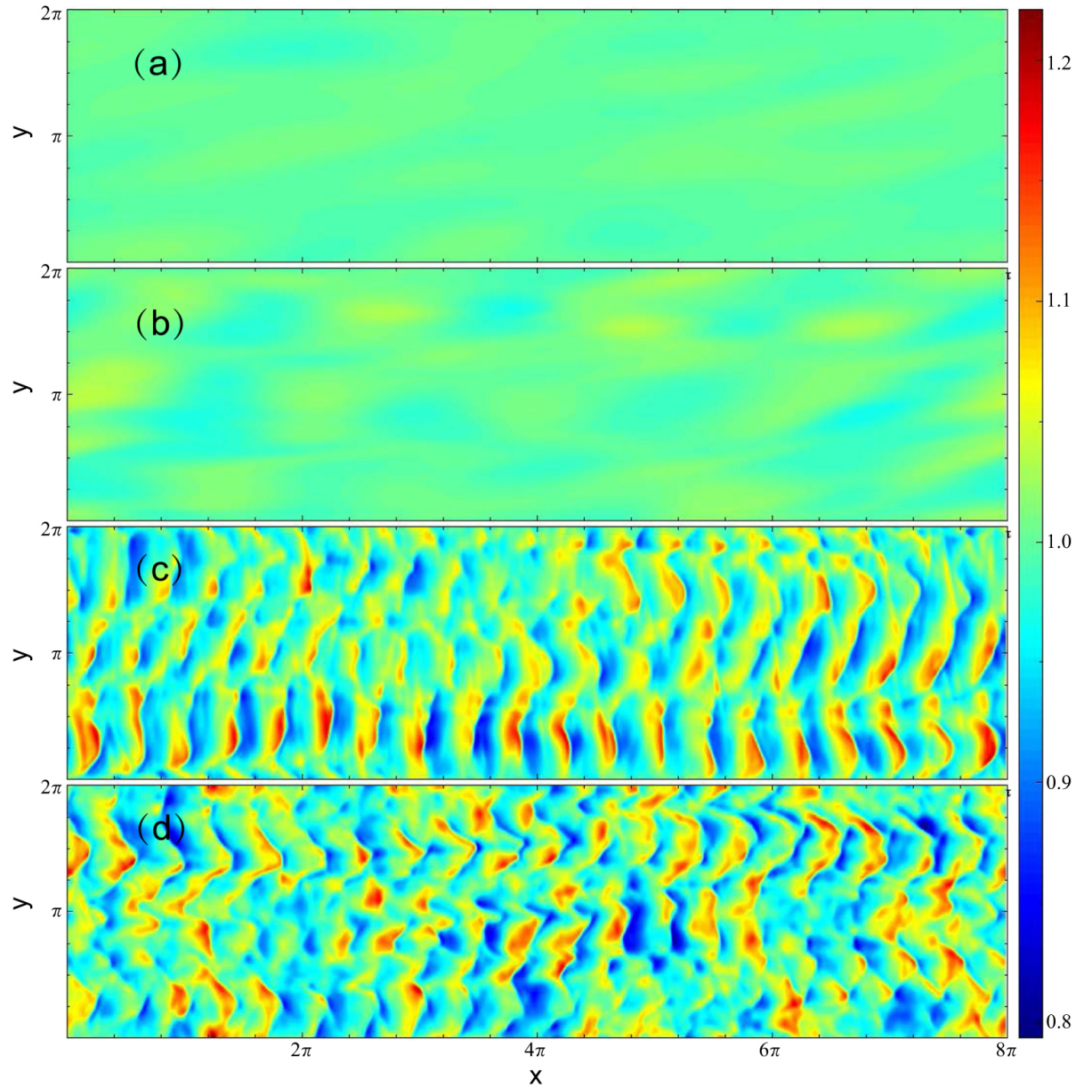
Figure 3. from The Parametric Decay Instability of Alfvén Waves in Turbulent Plasmas and the Applications in the Solar Wind null 2017 APJ 842 63 doi:10.3847/1538-4357/aa71b6 https://dx.doi.org/10.3847/1538-4357/aa71b6 © 2017. The American Astronomical Society. All rights reserved.
