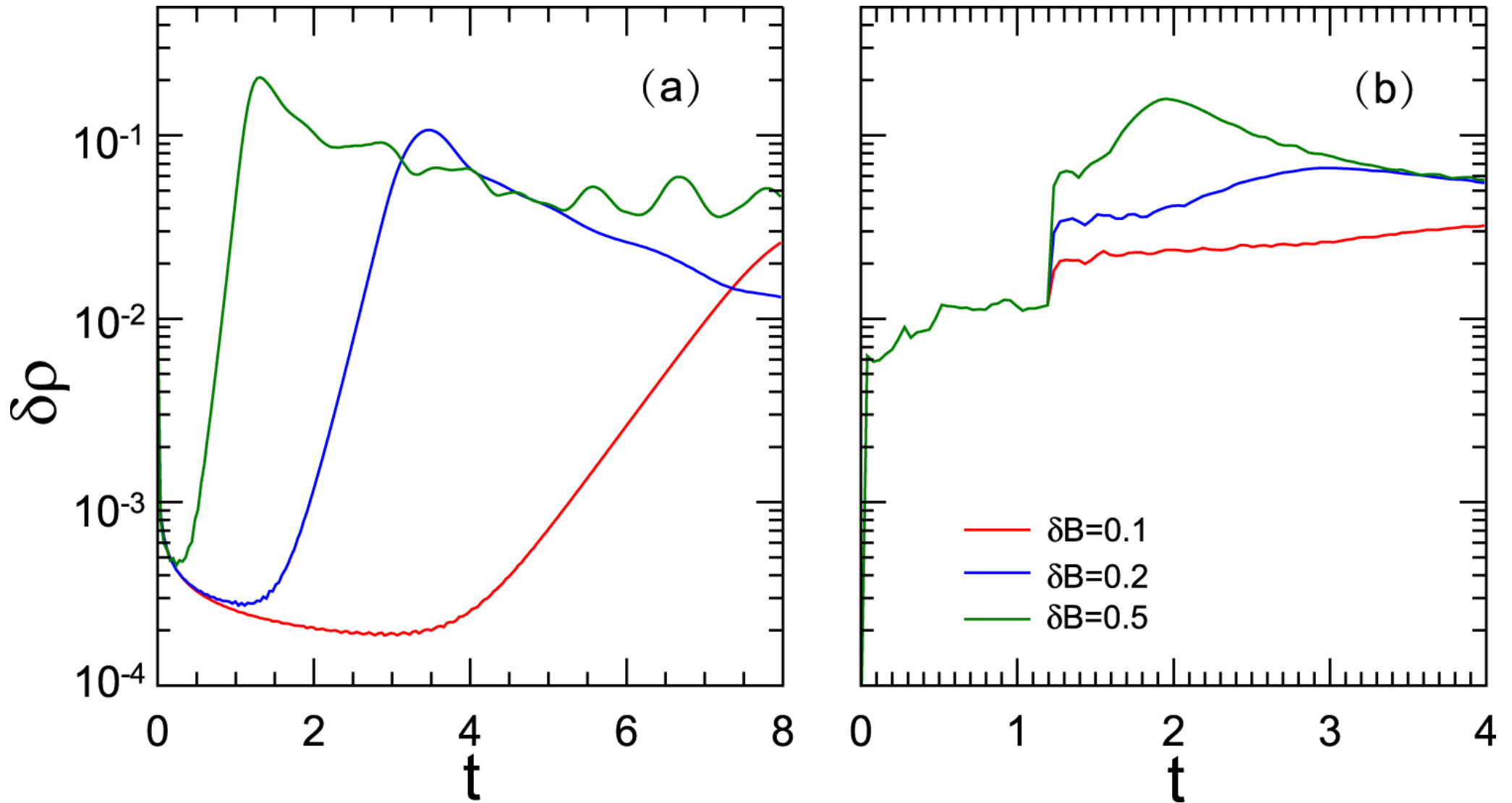
Figure 2. from The Parametric Decay Instability of Alfvén Waves in Turbulent Plasmas and the Applications in the Solar Wind null 2017 APJ 842 63 doi:10.3847/1538-4357/aa71b6 https://dx.doi.org/10.3847/1538-4357/aa71b6 © 2017. The American Astronomical Society. All rights reserved.
