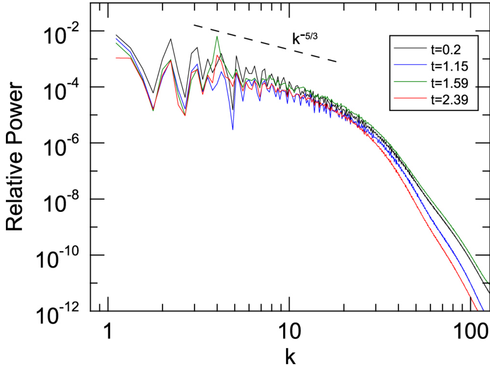
Figure 1. from The Parametric Decay Instability of Alfvén Waves in Turbulent Plasmas and the Applications in the Solar Wind null 2017 APJ 842 63 doi:10.3847/1538-4357/aa71b6 https://dx.doi.org/10.3847/1538-4357/aa71b6 © 2017. The American Astronomical Society. All rights reserved.
