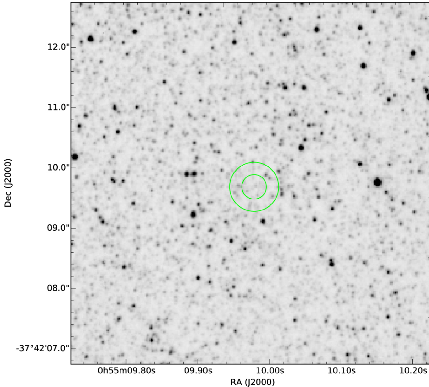
Figure 4. from Discovery of a Rapid, Luminous Nova in NGC 300 by the KMTNet Supernova Program null 2017 APJ 844 160 doi:10.3847/1538-4357/aa706b https://dx.doi.org/10.3847/1538-4357/aa706b © 2017. The American Astronomical Society. All rights reserved.
