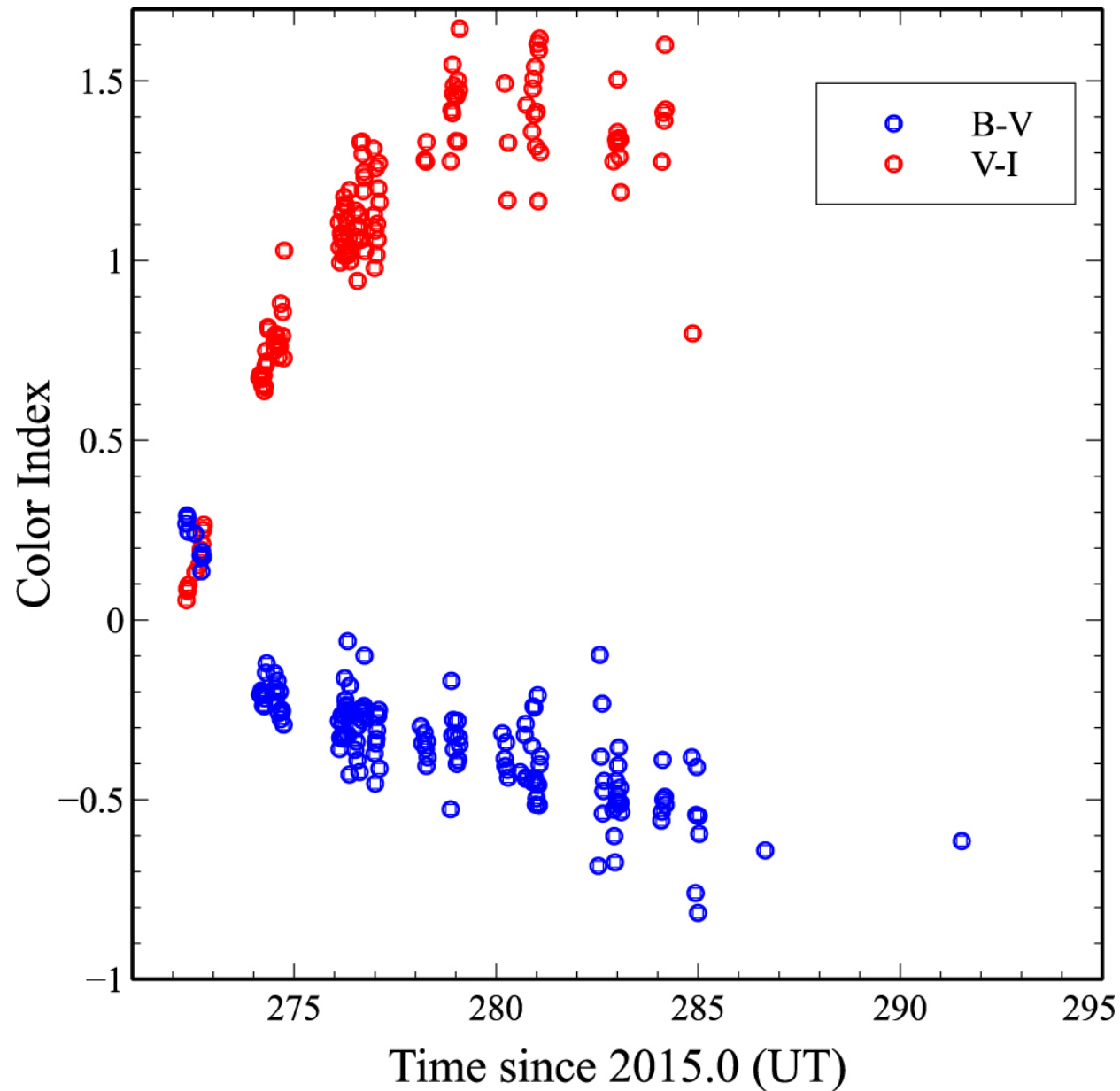
Figure 3. from Discovery of a Rapid, Luminous Nova in NGC 300 by the KMTNet Supernova Program null 2017 APJ 844 160 doi:10.3847/1538-4357/aa706b https://dx.doi.org/10.3847/1538-4357/aa706b © 2017. The American Astronomical Society. All rights reserved.
