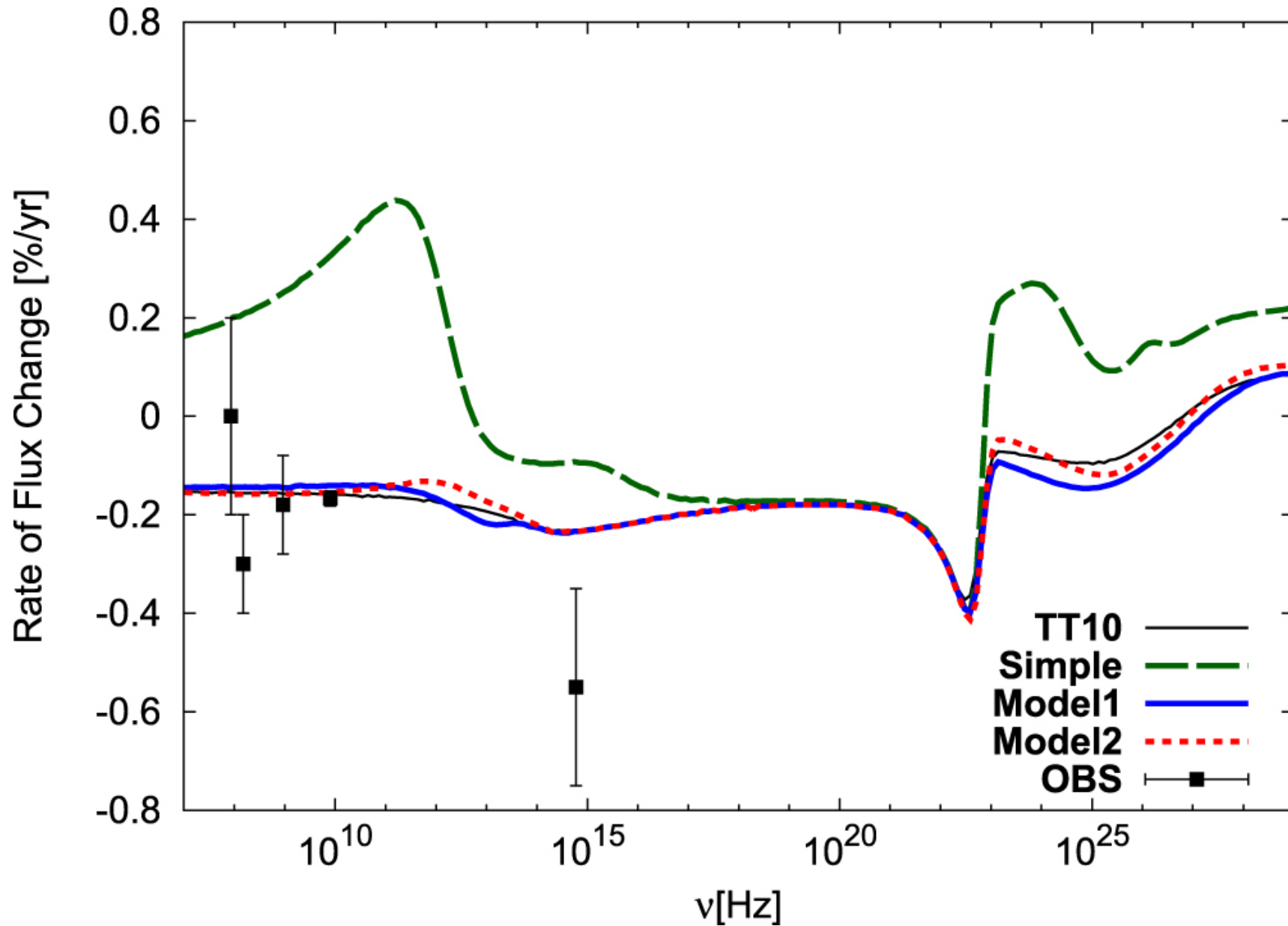
Figure 2. from On the Radio-emitting Particles of the Crab Nebula: Stochastic Acceleration Model null 2017 APJ 841 78 doi:10.3847/1538-4357/aa6f13 https://dx.doi.org/10.3847/1538-4357/aa6f13 © 2017. The American Astronomical Society. All rights reserved.
