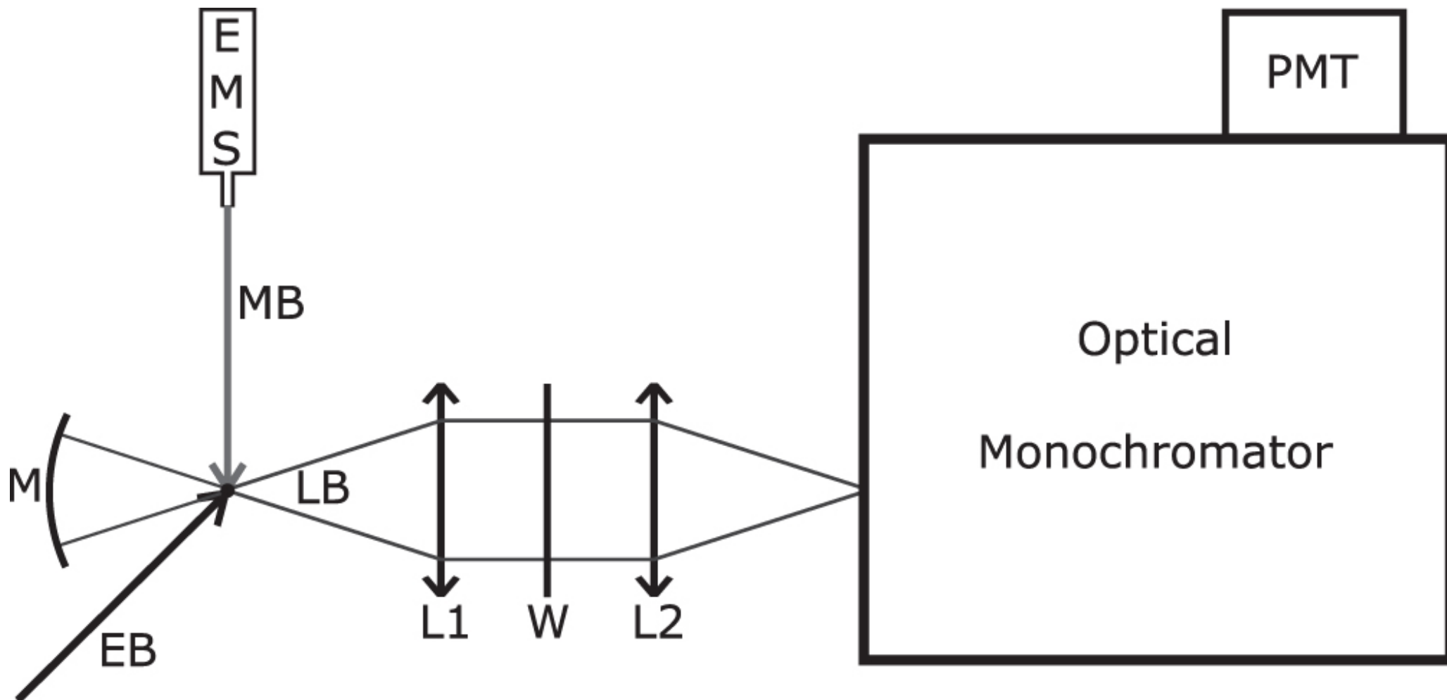
Figure 1. from Dissociative Excitation of Acetylene Induced by Electron Impact: Excitation-emission Cross-sections null 2017 APJ 841 17 doi:10.3847/1538-4357/aa6e54 https://dx.doi.org/10.3847/1538-4357/aa6e54 © 2017. The American Astronomical Society. All rights reserved.
