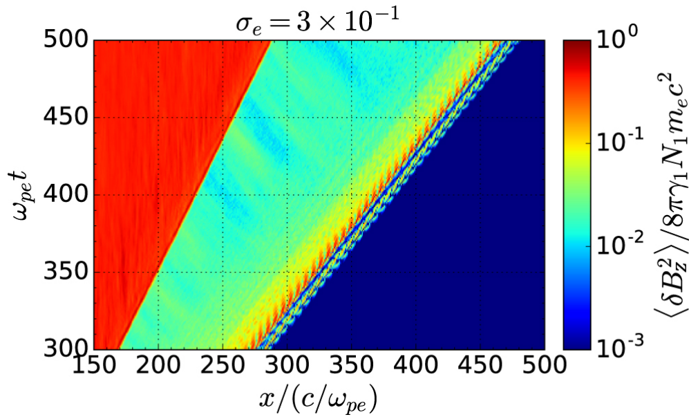
Figure 4. from Persistence of Precursor Waves in Two-dimensional Relativistic Shocks null 2017 APJ 840 52 doi:10.3847/1538-4357/aa6d6f https://dx.doi.org/10.3847/1538-4357/aa6d6f © 2017. The American Astronomical Society. All rights reserved.
