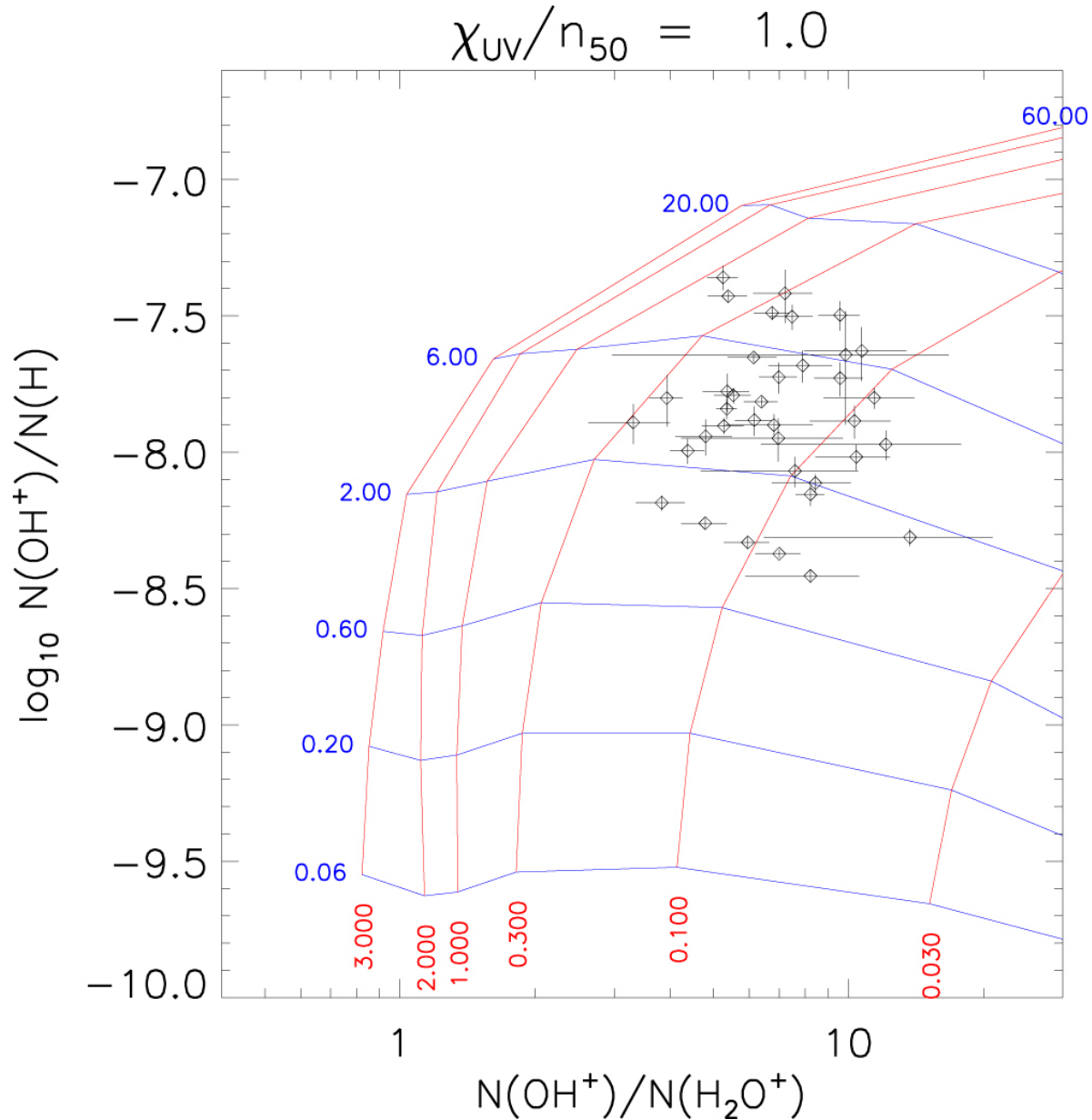
Figure 7. from The Cosmic-Ray Ionization Rate in the Galactic Disk, as Determined from Observations of Molecular Ions null 2017 APJ 845 163 doi:10.3847/1538-4357/aa6d68 https://dx.doi.org/10.3847/1538-4357/aa6d68 © 2017. The American Astronomical Society. All rights reserved.
