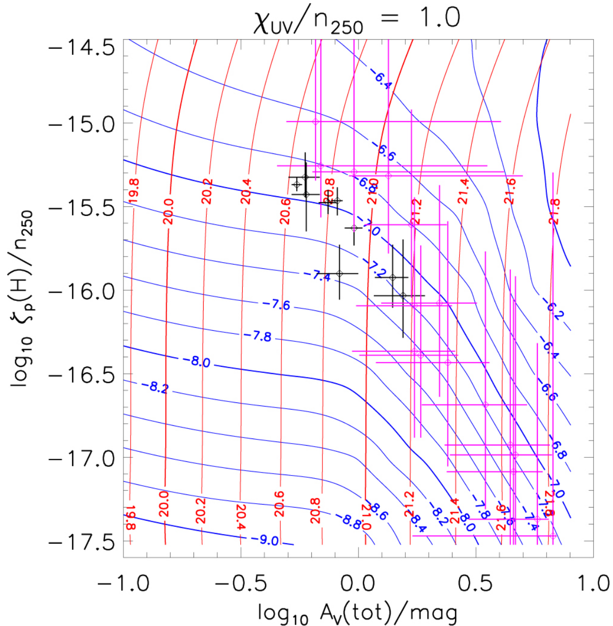
Figure 5. from The Cosmic-Ray Ionization Rate in the Galactic Disk, as Determined from Observations of Molecular Ions null 2017 APJ 845 163 doi:10.3847/1538-4357/aa6d68 https://dx.doi.org/10.3847/1538-4357/aa6d68 © 2017. The American Astronomical Society. All rights reserved.
