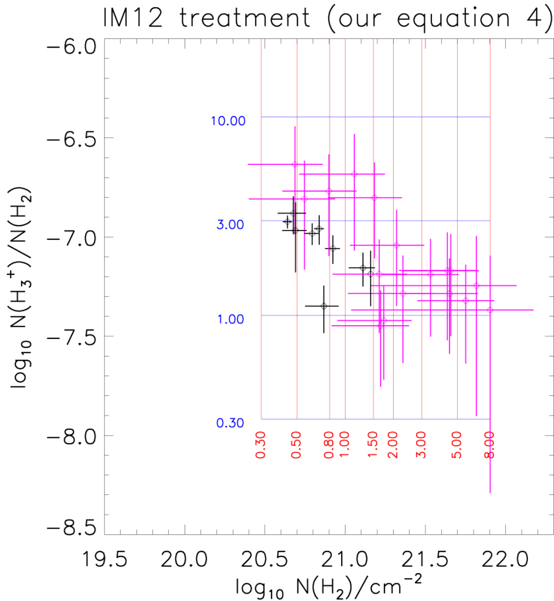
Figure 4. from The Cosmic-Ray Ionization Rate in the Galactic Disk, as Determined from Observations of Molecular Ions null 2017 APJ 845 163 doi:10.3847/1538-4357/aa6d68 https://dx.doi.org/10.3847/1538-4357/aa6d68 © 2017. The American Astronomical Society. All rights reserved.
