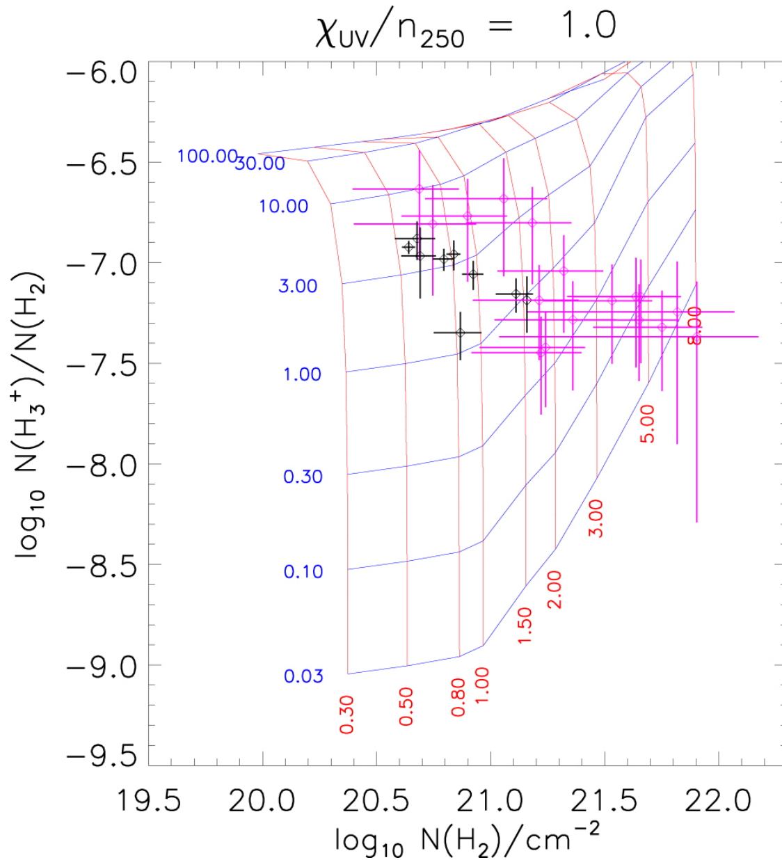
Figure 3. from The Cosmic-Ray Ionization Rate in the Galactic Disk, as Determined from Observations of Molecular Ions null 2017 APJ 845 163 doi:10.3847/1538-4357/aa6d68 https://dx.doi.org/10.3847/1538-4357/aa6d68 © 2017. The American Astronomical Society. All rights reserved.
