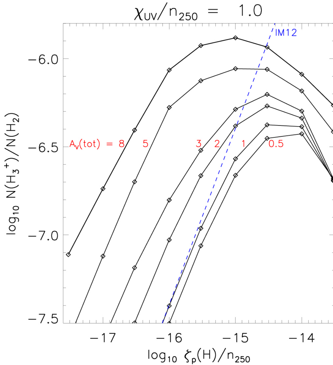
Figure 2. from The Cosmic-Ray Ionization Rate in the Galactic Disk, as Determined from Observations of Molecular Ions null 2017 APJ 845 163 doi:10.3847/1538-4357/aa6d68 https://dx.doi.org/10.3847/1538-4357/aa6d68 © 2017. The American Astronomical Society. All rights reserved.
