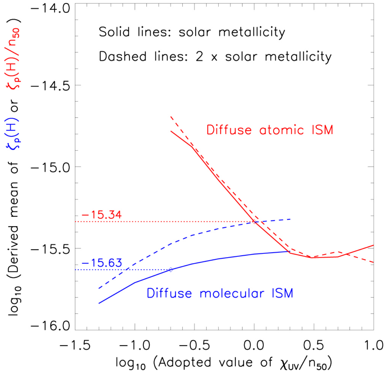
Figure 12. from The Cosmic-Ray Ionization Rate in the Galactic Disk, as Determined from Observations of Molecular Ions null 2017 APJ 845 163 doi:10.3847/1538-4357/aa6d68 https://dx.doi.org/10.3847/1538-4357/aa6d68 © 2017. The American Astronomical Society. All rights reserved.
