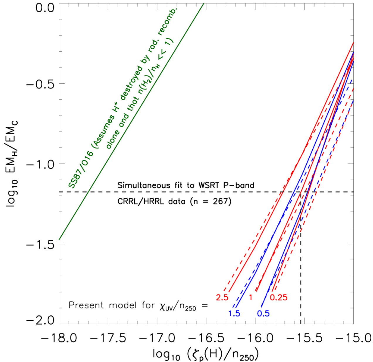
Figure 11. from The Cosmic-Ray Ionization Rate in the Galactic Disk, as Determined from Observations of Molecular Ions null 2017 APJ 845 163 doi:10.3847/1538-4357/aa6d68 https://dx.doi.org/10.3847/1538-4357/aa6d68
