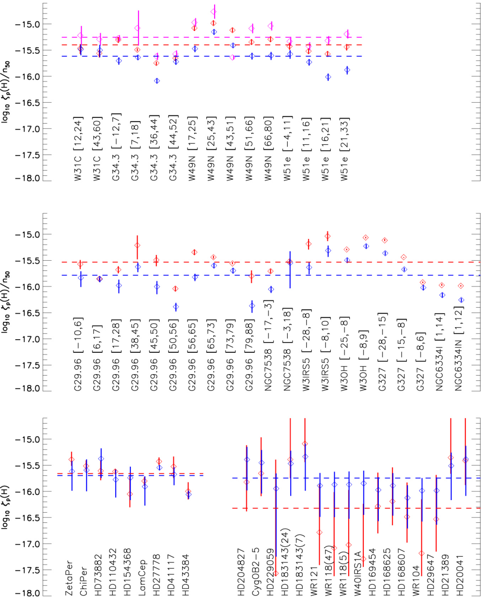
Figure 10. from The Cosmic-Ray Ionization Rate in the Galactic Disk, as Determined from Observations of Molecular Ions null 2017 APJ 845 163 doi:10.3847/1538-4357/aa6d68 https://dx.doi.org/10.3847/1538-4357/aa6d68 © 2017. The American Astronomical Society. All rights reserved.
