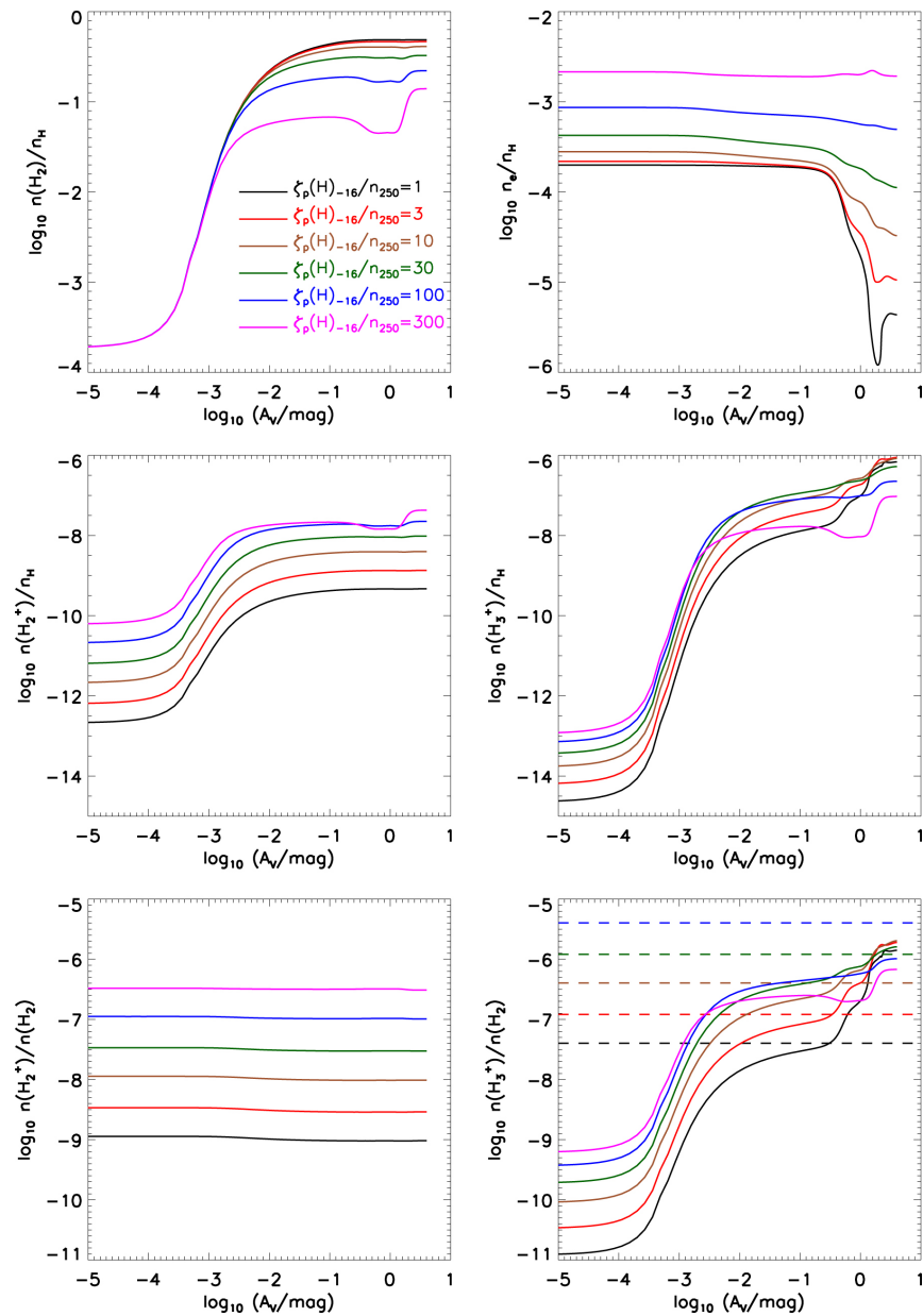
Figure 1. from The Cosmic-Ray Ionization Rate in the Galactic Disk, as Determined from Observations of Molecular Ions null 2017 APJ 845 163 doi:10.3847/1538-4357/aa6d68 https://dx.doi.org/10.3847/1538-4357/aa6d68
