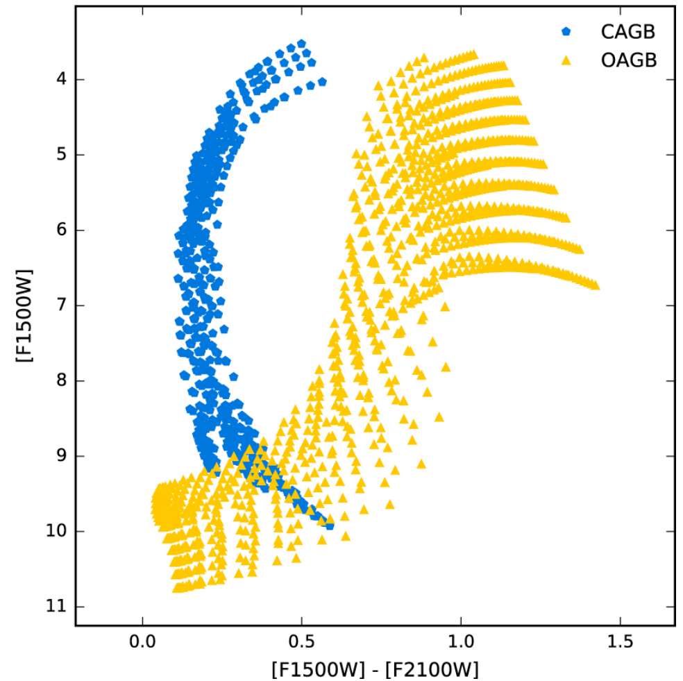
Figure 5. from Probing the Dusty Stellar Populations of the Local Volume Galaxies with JWST/MIRI null 2017 APJ 841 15 doi:10.3847/1538-4357/aa6bf6 https://dx.doi.org/10.3847/1538-4357/aa6bf6 © 2017. The American Astronomical Society. All rights reserved.
