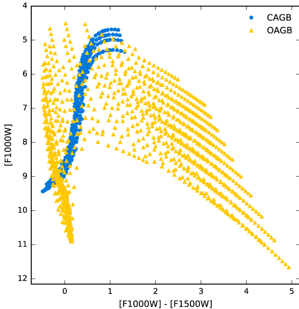
Figure 5. from Probing the Dusty Stellar Populations of the Local Volume Galaxies with JWST/MIRI null 2017 APJ 841 15 doi:10.3847/1538-4357/aa6bf6 https://dx.doi.org/10.3847/1538-4357/aa6bf6 © 2017. The American Astronomical Society. All rights reserved.
