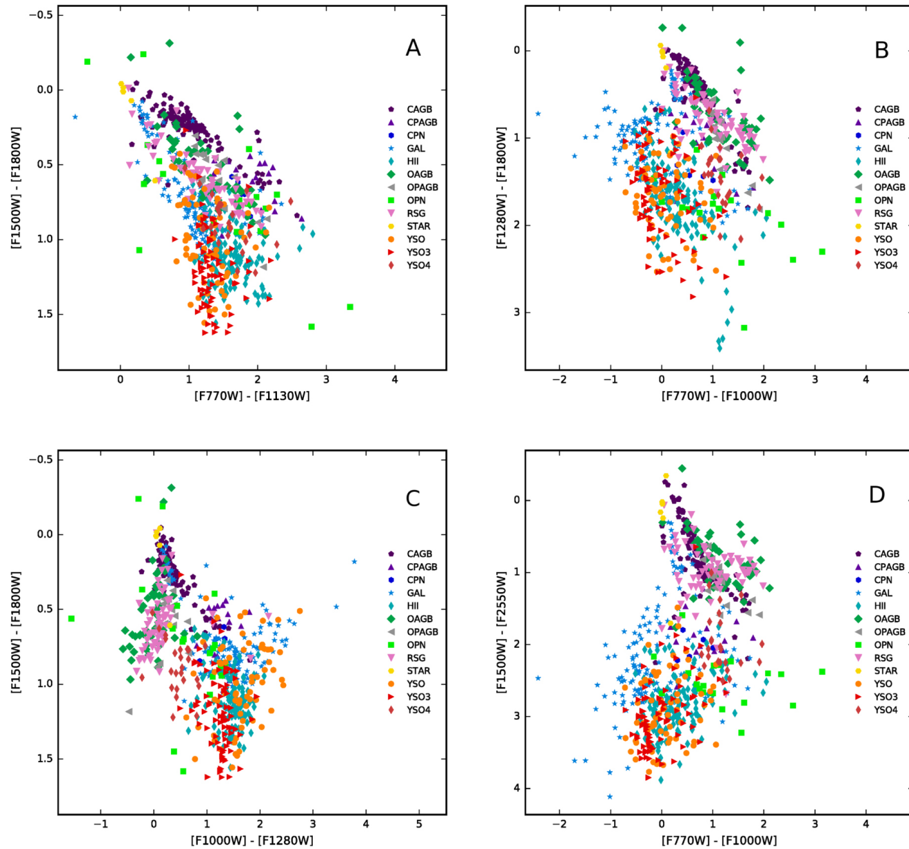
Figure 4. from Probing the Dusty Stellar Populations of the Local Volume Galaxies with JWST/MIRI null 2017 APJ 841 15 doi:10.3847/1538-4357/aa6bf6 https://dx.doi.org/10.3847/1538-4357/aa6bf6 © 2017. The American Astronomical Society. All rights reserved.
