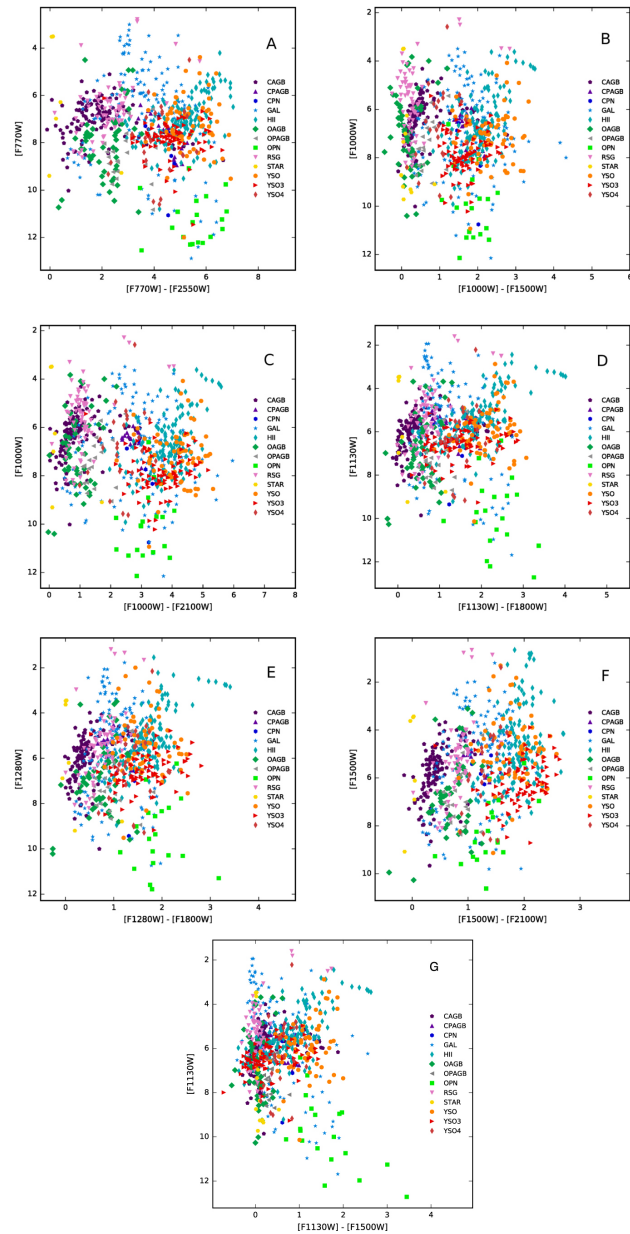
Figure 3. from Probing the Dusty Stellar Populations of the Local Volume Galaxies with JWST/MIRI null 2017 APJ 841 15 doi:10.3847/1538-4357/aa6bf6 https://dx.doi.org/10.3847/1538-4357/aa6bf6 © 2017. The American Astronomical Society. All rights reserved.
