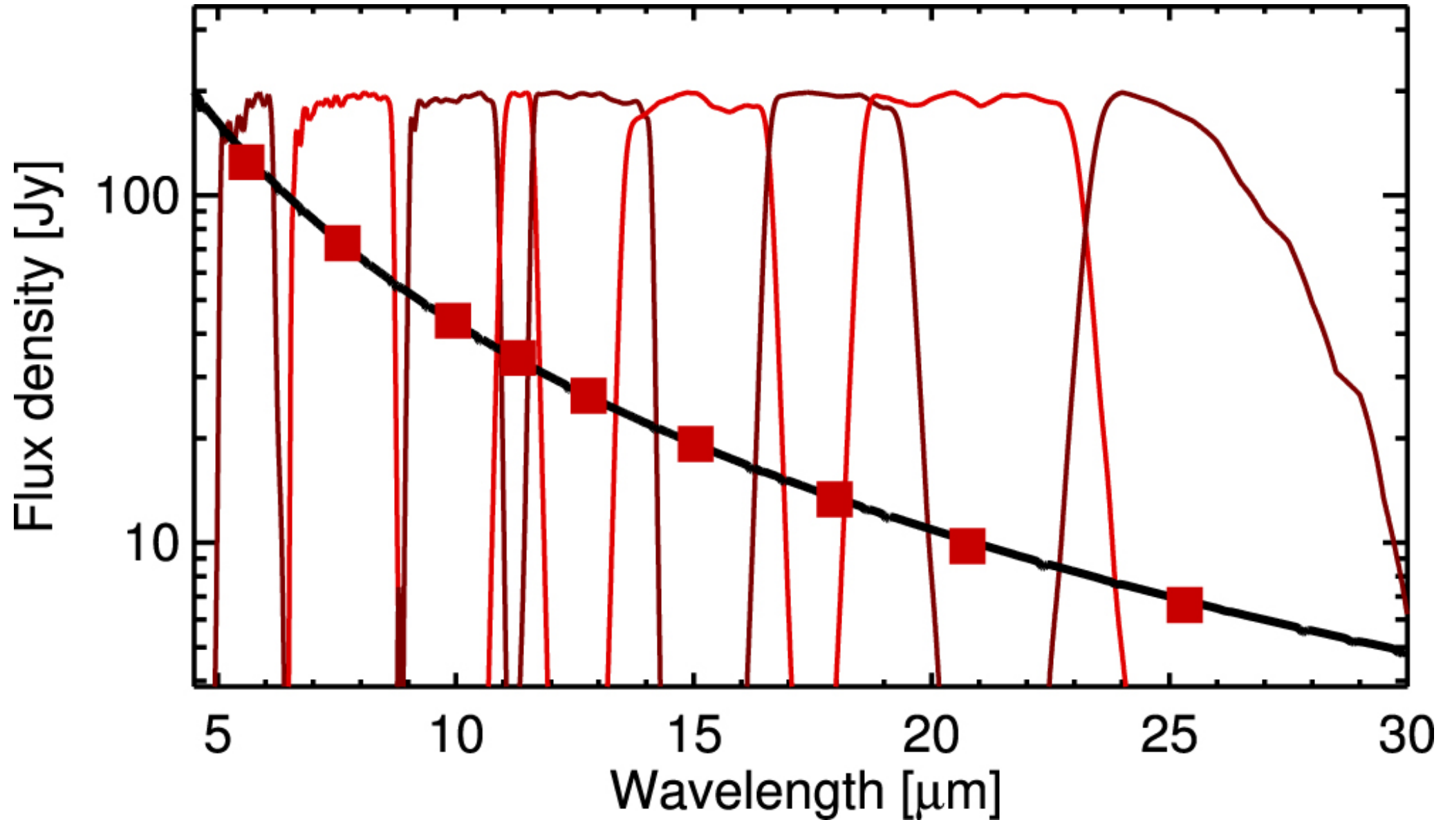
Figure 2. from Probing the Dusty Stellar Populations of the Local Volume Galaxies with JWST/MIRI null 2017 APJ 841 15 doi:10.3847/1538-4357/aa6bf6 https://dx.doi.org/10.3847/1538-4357/aa6bf6 © 2017. The American Astronomical Society. All rights reserved.
