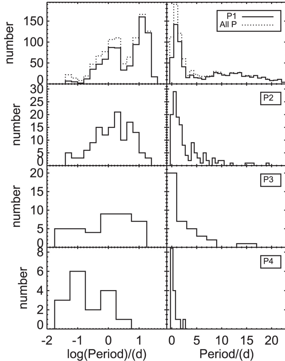
Figure 5. from Rotation of Late-type Stars in Praesepe with K2 null 2017 APJ 839 92 doi:10.3847/1538-4357/aa6aa4 https://dx.doi.org/10.3847/1538-4357/aa6aa4 © 2017. The American Astronomical Society. All rights reserved.
