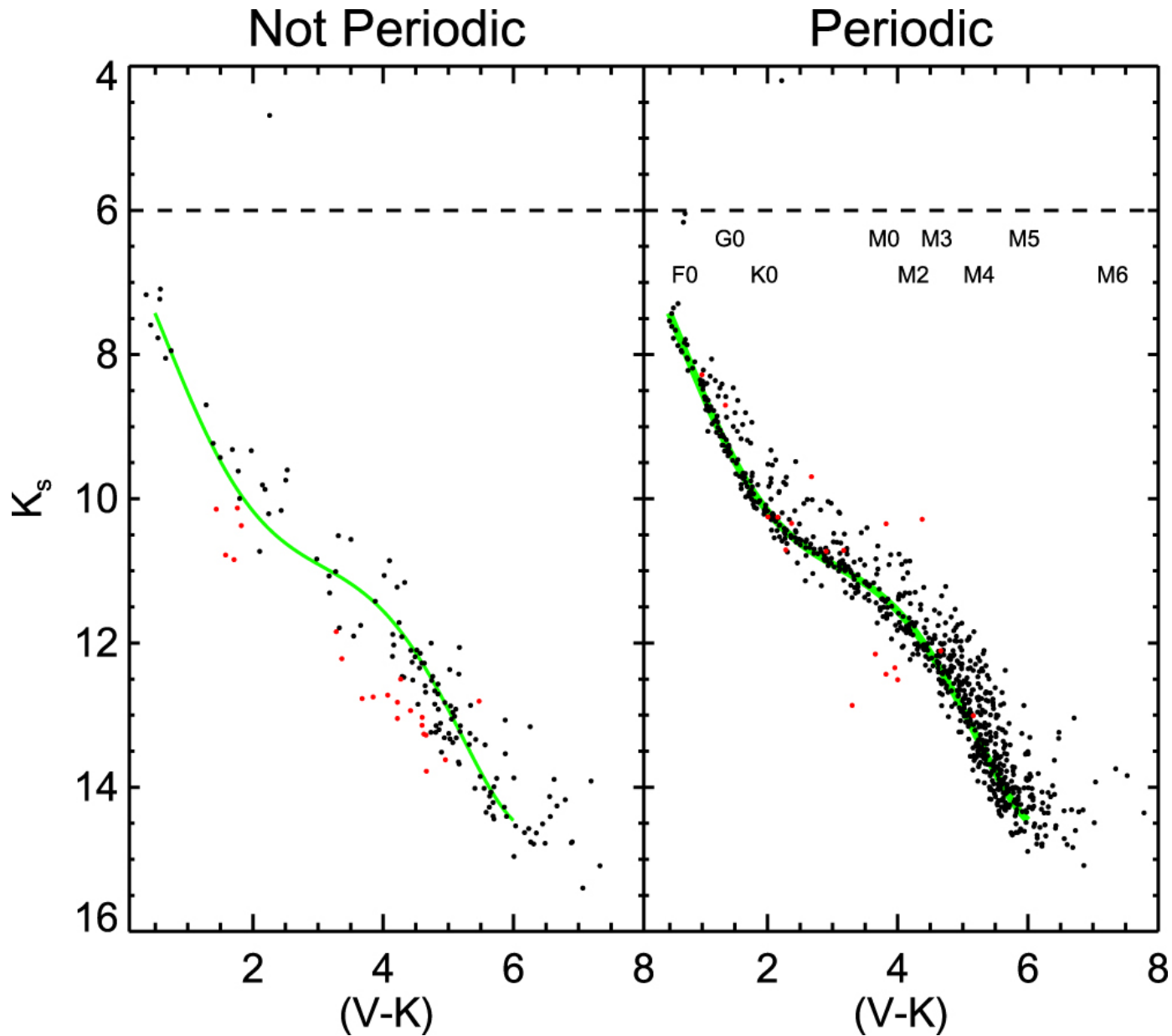
Figure 4. from Rotation of Late-type Stars in Praesepe with K2 null 2017 APJ 839 92 doi:10.3847/1538-4357/aa6aa4 https://dx.doi.org/10.3847/1538-4357/aa6aa4 © 2017. The American Astronomical Society. All rights reserved.
