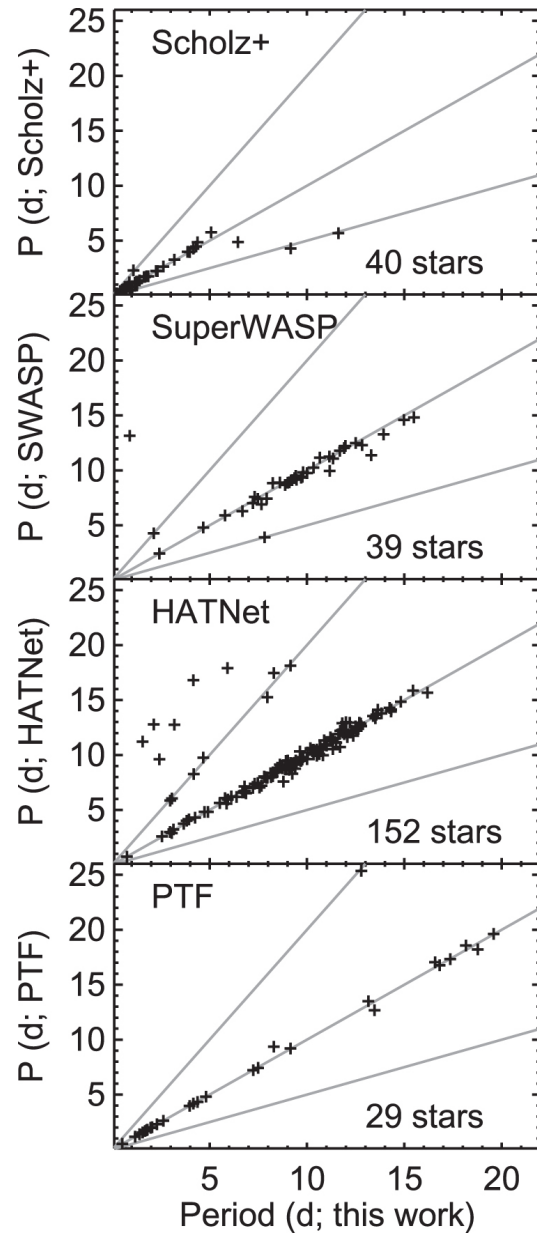
Figure 3. from Rotation of Late-type Stars in Praesepe with K2 null 2017 APJ 839 92 doi:10.3847/1538-4357/aa6aa4 https://dx.doi.org/10.3847/1538-4357/aa6aa4 © 2017. The American Astronomical Society. All rights reserved.
