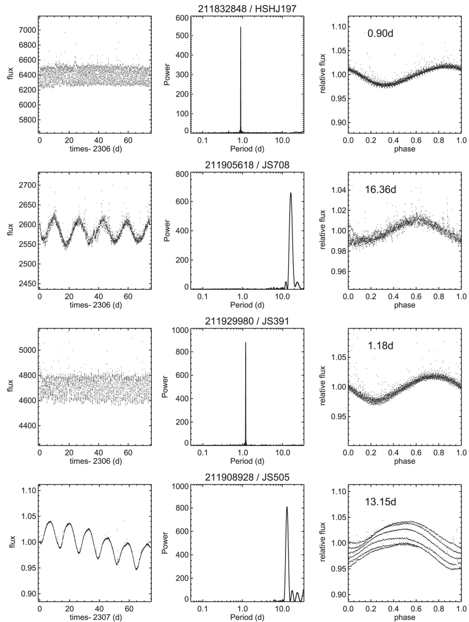
Figure 2. from Rotation of Late-type Stars in Praesepe with K2 null 2017 APJ 839 92 doi:10.3847/1538-4357/aa6aa4 https://dx.doi.org/10.3847/1538-4357/aa6aa4 © 2017. The American Astronomical Society. All rights reserved.
