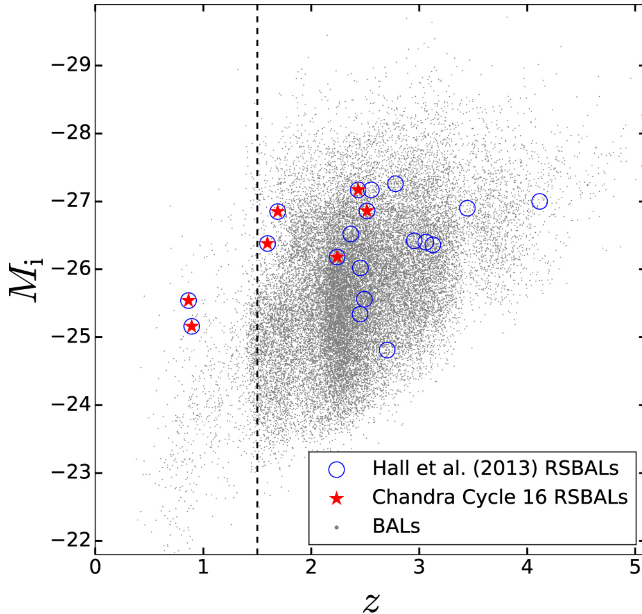
Figure 2. from X-Ray Insights into the Nature of Quasars with Redshifted Broad Absorption Lines null 2017 APJ 839 101 doi:10.3847/1538-4357/aa6842 https://dx.doi.org/10.3847/1538-4357/aa6842 © 2017. The American Astronomical Society. All rights reserved.
