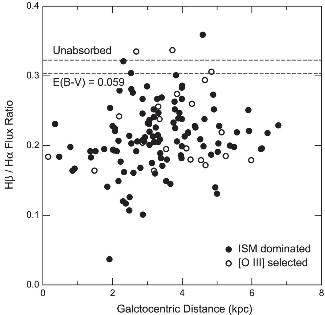
Figure 7. from A Spectroscopic Study of the Rich Supernova Remnant Population in M83 null 2017 APJ 839 83 doi:10.3847/1538-4357/aa683d https://dx.doi.org/10.3847/1538-4357/aa683d © 2017. The American Astronomical Society. All rights reserved.
