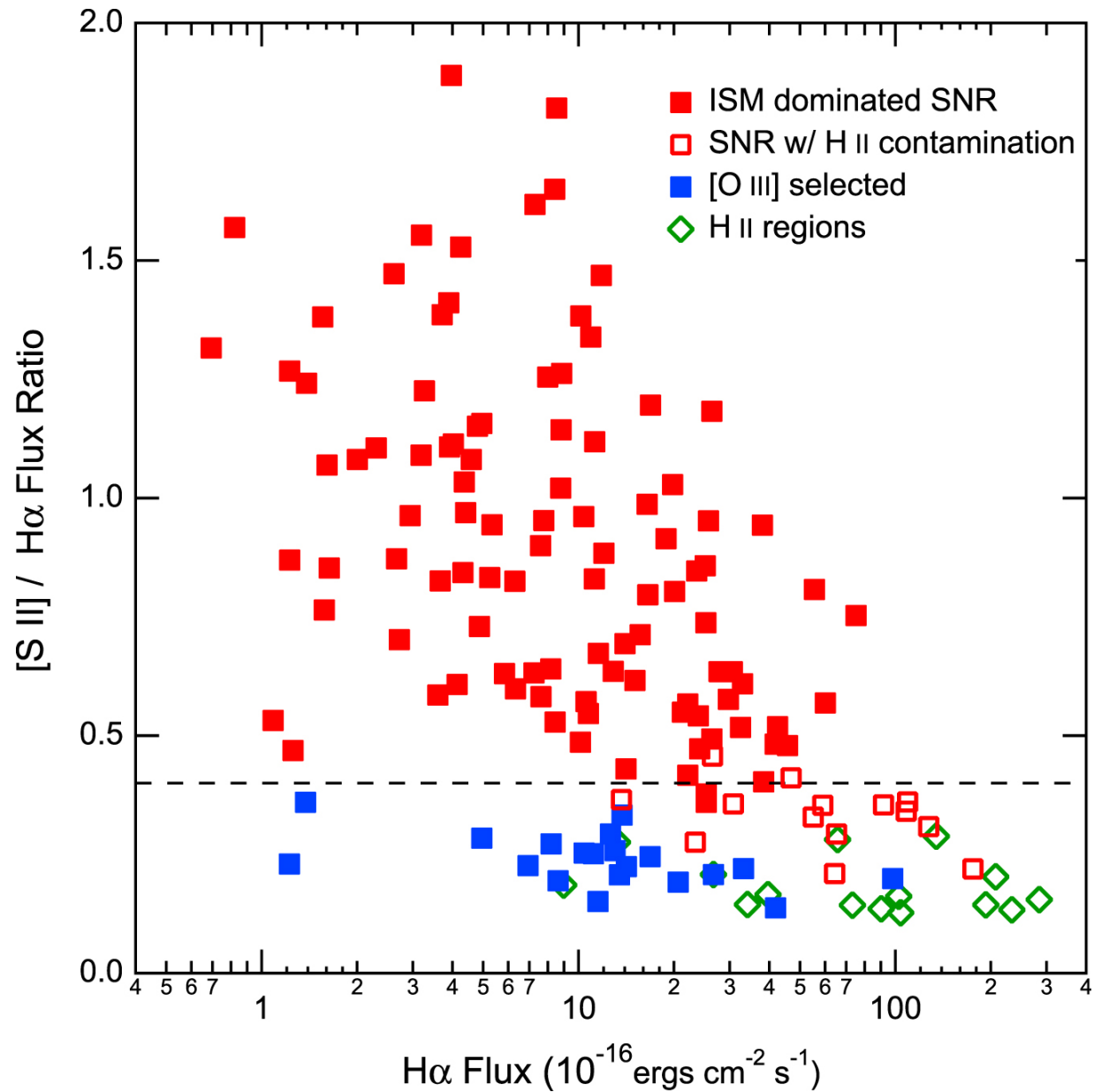
Figure 6. from A Spectroscopic Study of the Rich Supernova Remnant Population in M83 null 2017 APJ 839 83 doi:10.3847/1538-4357/aa683d https://dx.doi.org/10.3847/1538-4357/aa683d © 2017. The American Astronomical Society. All rights reserved.
