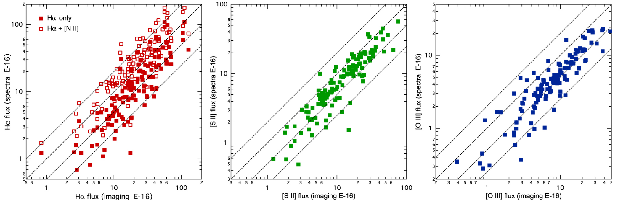
Figure 5. from A Spectroscopic Study of the Rich Supernova Remnant Population in M83 null 2017 APJ 839 83 doi:10.3847/1538-4357/aa683d https://dx.doi.org/10.3847/1538-4357/aa683d © 2017. The American Astronomical Society. All rights reserved.
