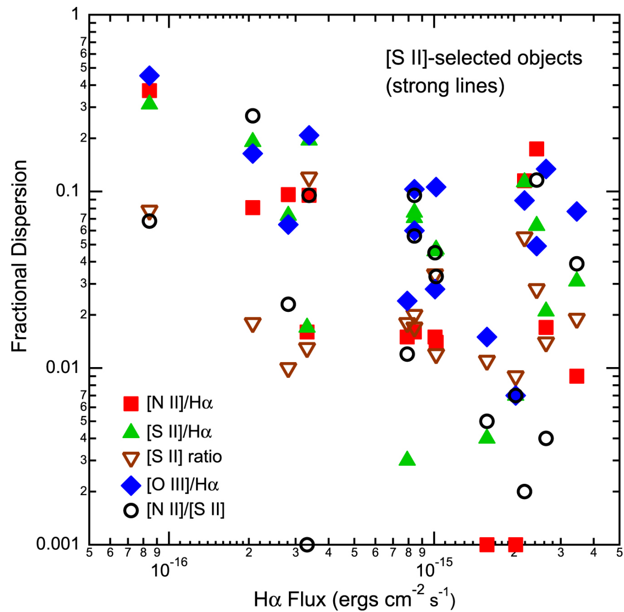
Figure 4. from A Spectroscopic Study of the Rich Supernova Remnant Population in M83 null 2017 APJ 839 83 doi:10.3847/1538-4357/aa683d https://dx.doi.org/10.3847/1538-4357/aa683d © 2017. The American Astronomical Society. All rights reserved.
