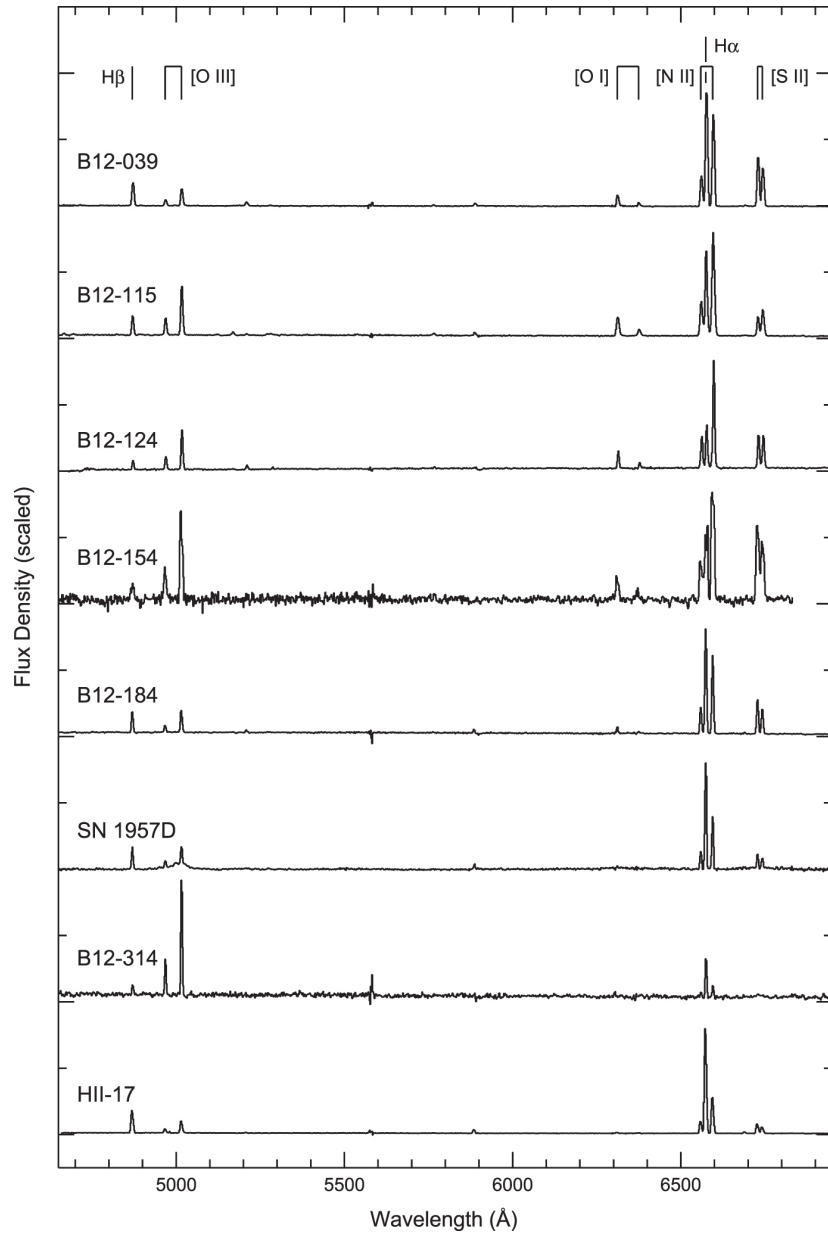
Figure 3. from A Spectroscopic Study of the Rich Supernova Remnant Population in M83 null 2017 APJ 839 83 doi:10.3847/1538-4357/aa683d https://dx.doi.org/10.3847/1538-4357/aa683d © 2017. The American Astronomical Society. All rights reserved.
