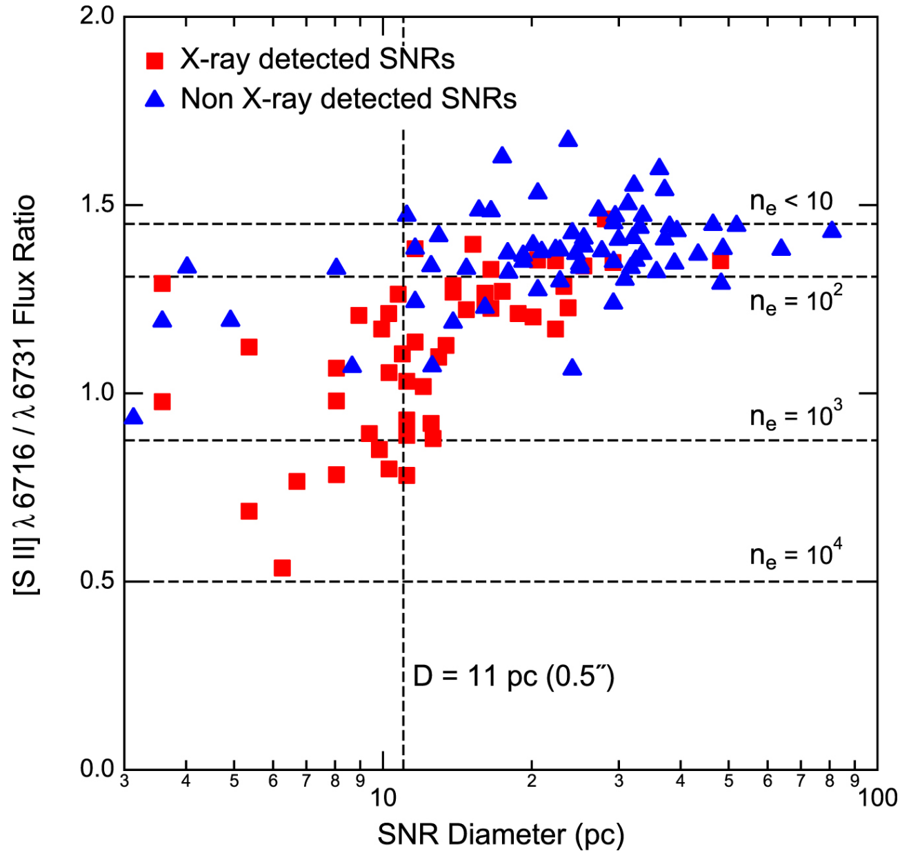
Figure 12. from A Spectroscopic Study of the Rich Supernova Remnant Population in M83 null 2017 APJ 839 83 doi:10.3847/1538-4357/aa683d https://dx.doi.org/10.3847/1538-4357/aa683d © 2017. The American Astronomical Society. All rights reserved.
