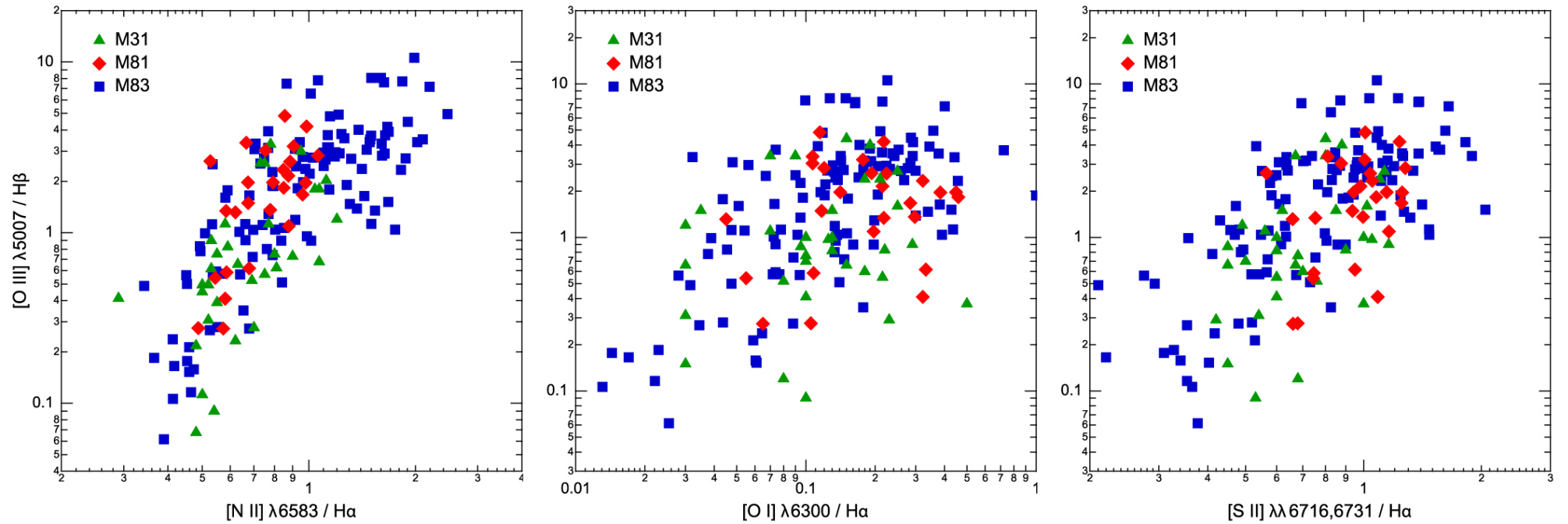
Figure 10. from A Spectroscopic Study of the Rich Supernova Remnant Population in M83 null 2017 APJ 839 83 doi:10.3847/1538-4357/aa683d https://dx.doi.org/10.3847/1538-4357/aa683d © 2017. The American Astronomical Society. All rights reserved.
