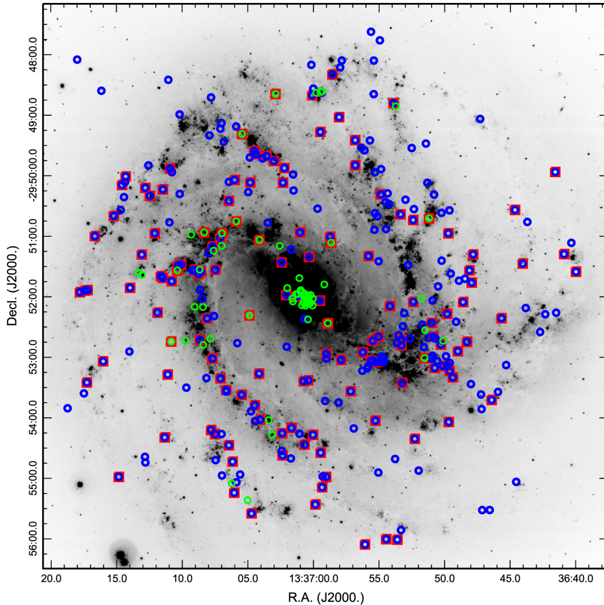
Figure 1. from A Spectroscopic Study of the Rich Supernova Remnant Population in M83 null 2017 APJ 839 83 doi:10.3847/1538-4357/aa683d https://dx.doi.org/10.3847/1538-4357/aa683d © 2017. The American Astronomical Society. All rights reserved.
