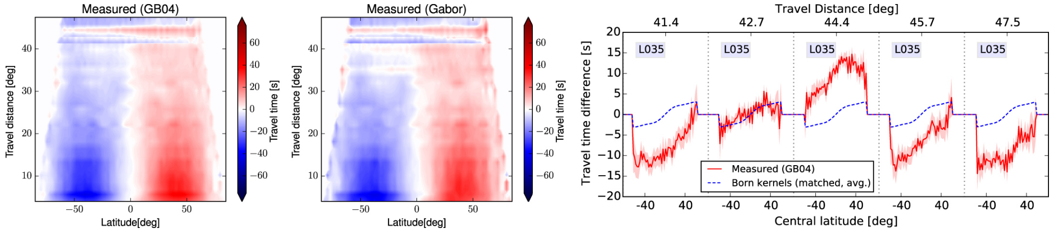
Figure 7. from Validation of Spherical Born Approximation Sensitivity Functions for Measuring Deep Solar Meridional Flow null 2017 APJ 838 53 doi:10.3847/1538-4357/aa6333 https://dx.doi.org/10.3847/1538-4357/aa6333 © 2017. The American Astronomical Society. All rights reserved.
