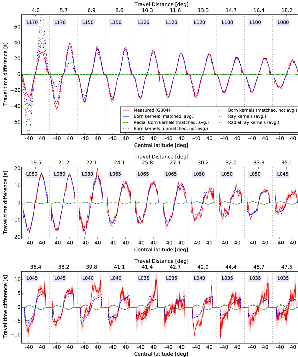
Figure 6. from Validation of Spherical Born Approximation Sensitivity Functions for Measuring Deep Solar Meridional Flow null 2017 APJ 838 53 doi:10.3847/1538-4357/aa6333 https://dx.doi.org/10.3847/1538-4357/aa6333 © 2017. The American Astronomical Society. All rights reserved.
