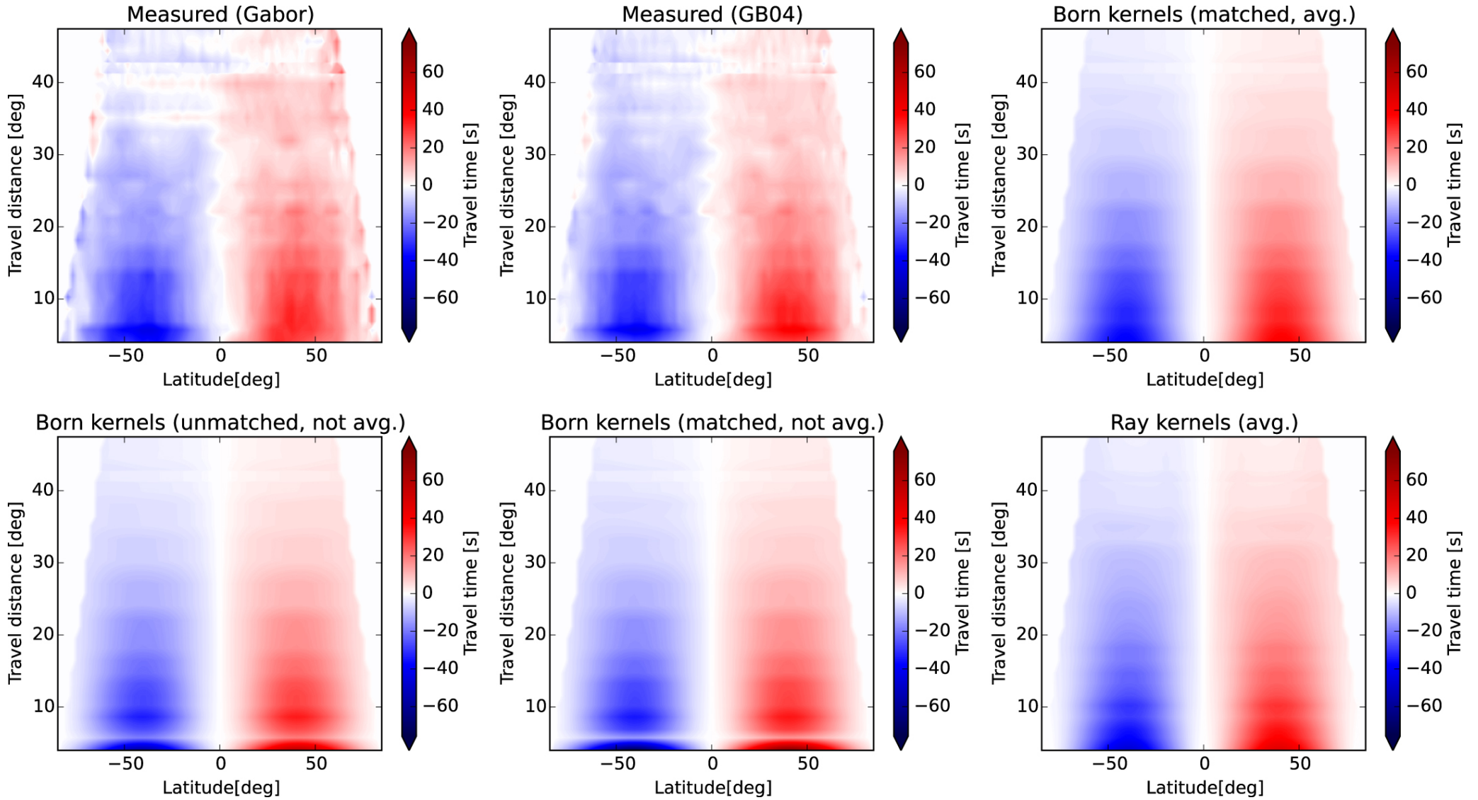
Figure 5. from Validation of Spherical Born Approximation Sensitivity Functions for Measuring Deep Solar Meridional Flow null 2017 APJ 838 53 doi:10.3847/1538-4357/aa6333 https://dx.doi.org/10.3847/1538-4357/aa6333 © 2017. The American Astronomical Society. All rights reserved.
