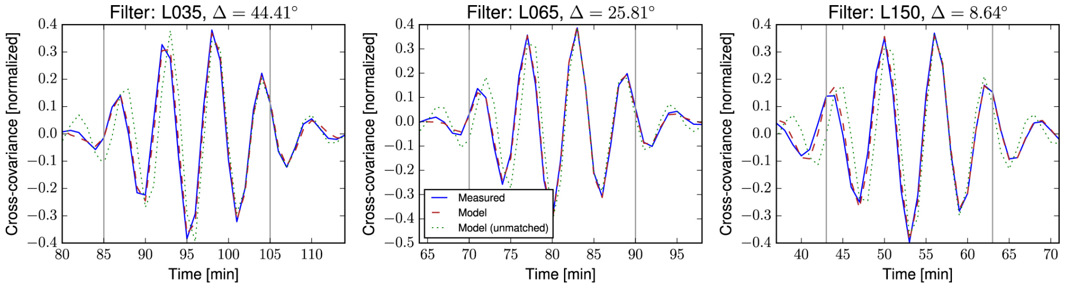
Figure 4. from Validation of Spherical Born Approximation Sensitivity Functions for Measuring Deep Solar Meridional Flow null 2017 APJ 838 53 doi:10.3847/1538-4357/aa6333 https://dx.doi.org/10.3847/1538-4357/aa6333 © 2017. The American Astronomical Society. All rights reserved.
