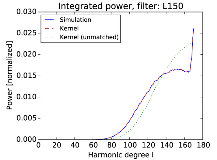
Figure 3. from Validation of Spherical Born Approximation Sensitivity Functions for Measuring Deep Solar Meridional Flow null 2017 APJ 838 53 doi:10.3847/1538-4357/aa6333 https://dx.doi.org/10.3847/1538-4357/aa6333 © 2017. The American Astronomical Society. All rights reserved.
