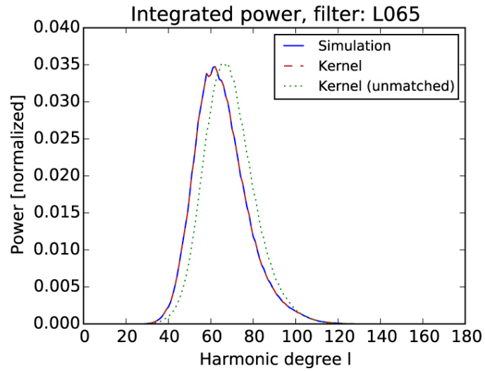
Figure 3. from Validation of Spherical Born Approximation Sensitivity Functions for Measuring Deep Solar Meridional Flow null 2017 APJ 838 53 doi:10.3847/1538-4357/aa6333 https://dx.doi.org/10.3847/1538-4357/aa6333 © 2017. The American Astronomical Society. All rights reserved.
