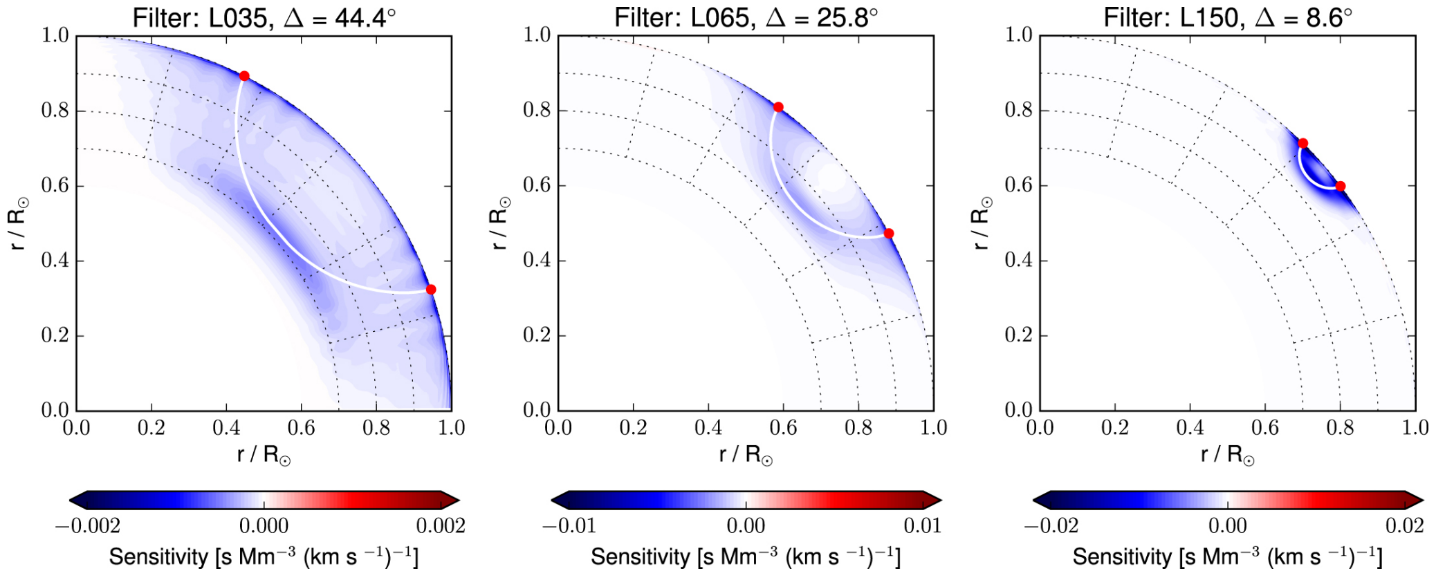
Figure 1. from Validation of Spherical Born Approximation Sensitivity Functions for Measuring Deep Solar Meridional Flow null 2017 APJ 838 53 doi:10.3847/1538-4357/aa6333 https://dx.doi.org/10.3847/1538-4357/aa6333 © 2017. The American Astronomical Society. All rights reserved.
