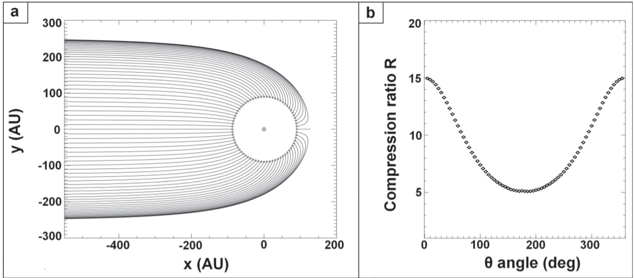
Figure 3. from Modeling the Plasma Flow in the Inner Heliosheath with a Spatially Varying Compression Ratio null 2017 APJ 838 7 doi:10.3847/1538-4357/aa61ff https://dx.doi.org/10.3847/1538-4357/aa61ff © 2017. The American Astronomical Society. All rights reserved.
