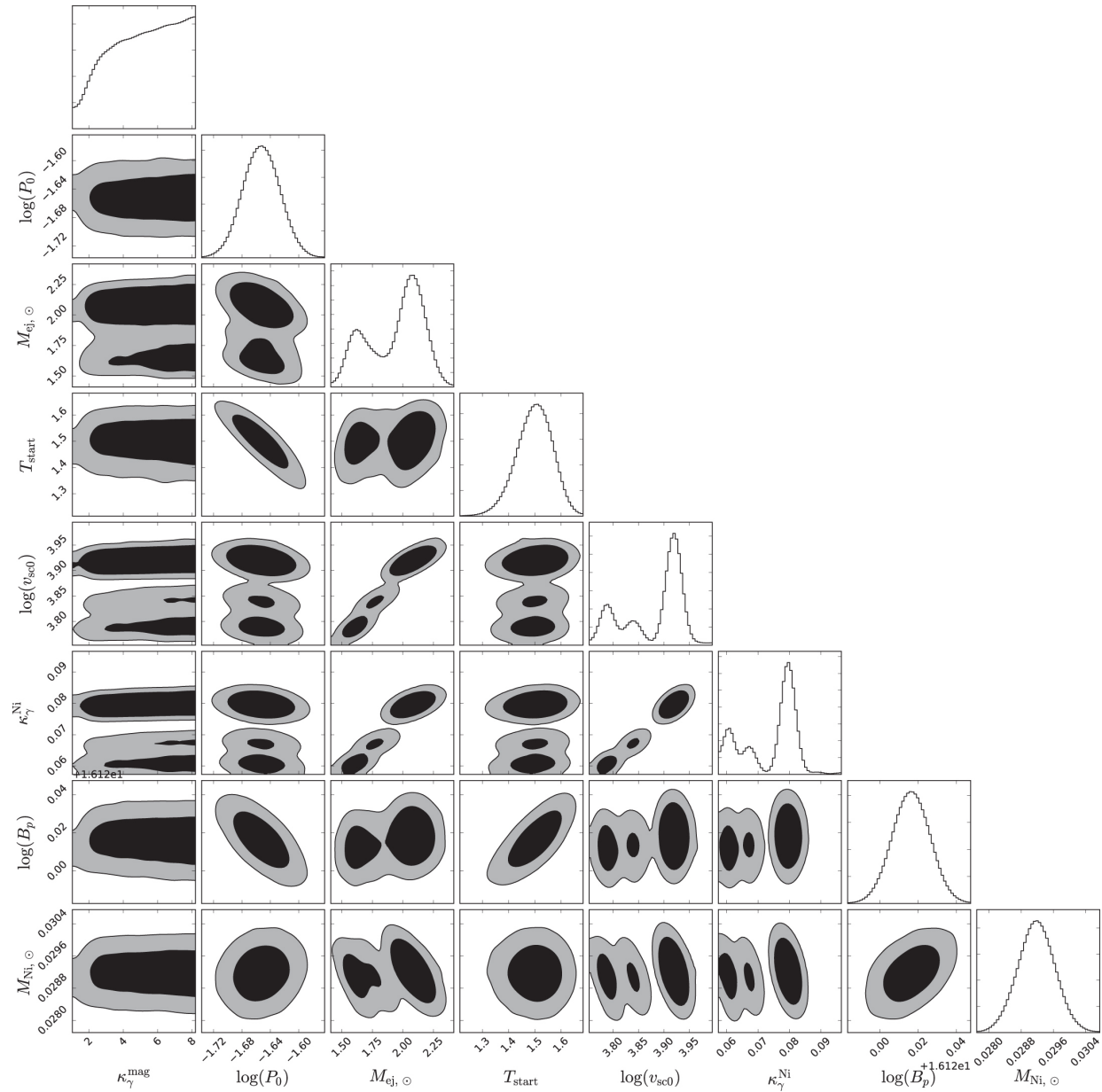
Figure 4. from Evidence for Magnetar Formation in Broad-lined Type Ic Supernovae 1998bw and 2002ap null 2017 APJ 837 128 doi:10.3847/1538-4357/aa5ff5 https://dx.doi.org/10.3847/1538-4357/aa5ff5 © 2017. The American Astronomical Society. All rights reserved.
