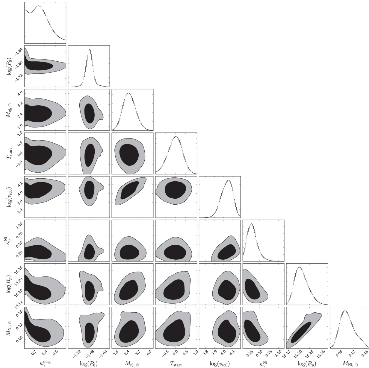
Figure 3. from Evidence for Magnetar Formation in Broad-lined Type Ic Supernovae 1998bw and 2002ap null 2017 APJ 837 128 doi:10.3847/1538-4357/aa5ff5 https://dx.doi.org/10.3847/1538-4357/aa5ff5 © 2017. The American Astronomical Society. All rights reserved.
