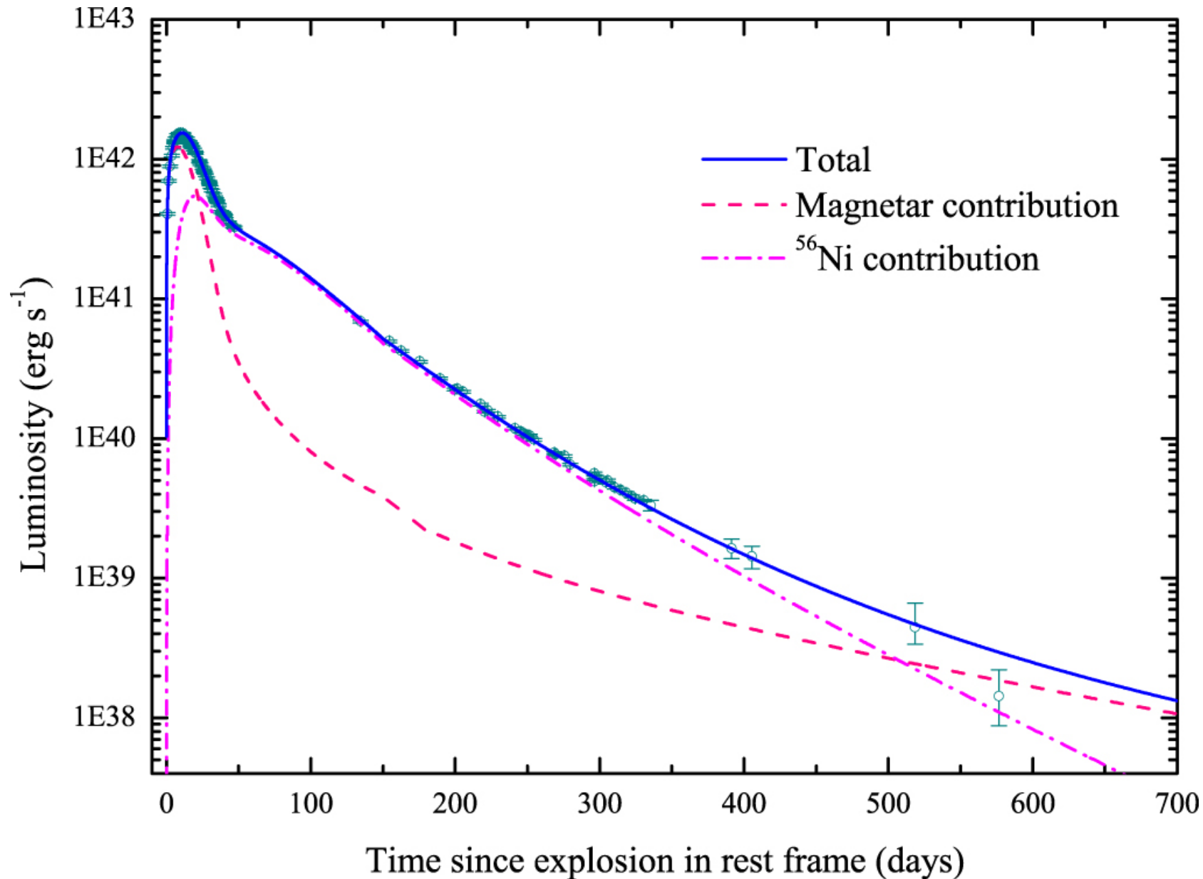
Figure 2. from Evidence for Magnetar Formation in Broad-lined Type Ic Supernovae 1998bw and 2002ap null 2017 APJ 837 128 doi:10.3847/1538-4357/aa5ff5 https://dx.doi.org/10.3847/1538-4357/aa5ff5 © 2017. The American Astronomical Society. All rights reserved.
