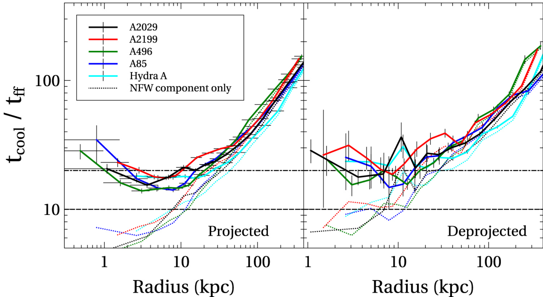
Figure 9. from Mass Distribution in Galaxy Cluster Cores null 2017 APJ 837 51 doi:10.3847/1538-4357/aa5f56 https://dx.doi.org/10.3847/1538-4357/aa5f56 © 2017. The American Astronomical Society. All rights reserved.
