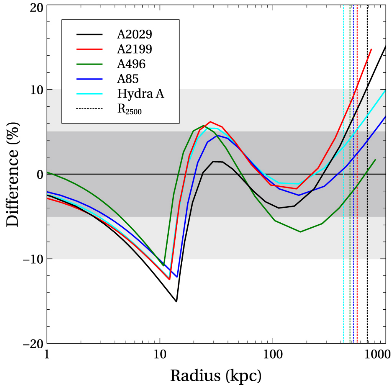
Figure 7. from Mass Distribution in Galaxy Cluster Cores null 2017 APJ 837 51 doi:10.3847/1538-4357/aa5f56 https://dx.doi.org/10.3847/1538-4357/aa5f56 © 2017. The American Astronomical Society. All rights reserved.
