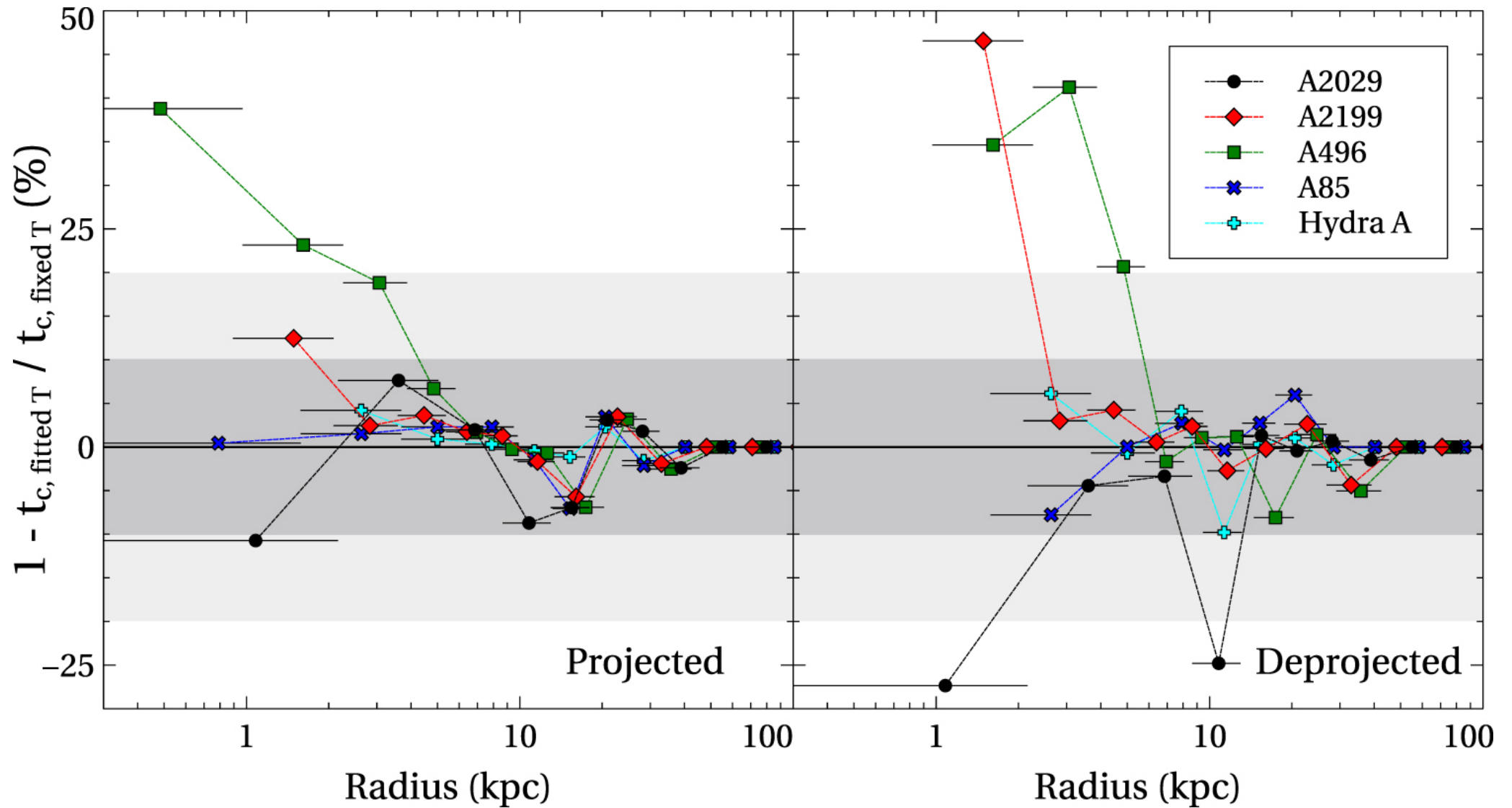
Figure 4. from Mass Distribution in Galaxy Cluster Cores null 2017 APJ 837 51 doi:10.3847/1538-4357/aa5f56 https://dx.doi.org/10.3847/1538-4357/aa5f56 © 2017. The American Astronomical Society. All rights reserved.
